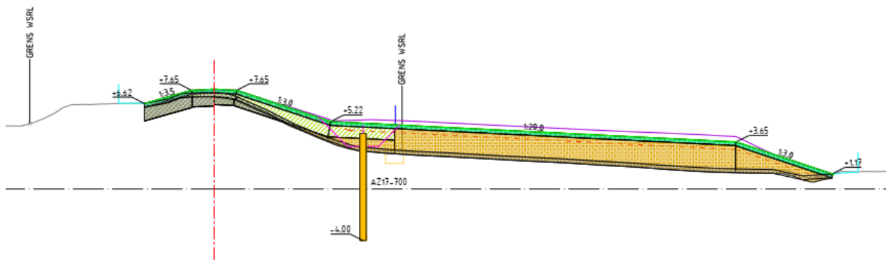
Figure 34: Reinforcement of the alternative landwards with soil (cross section TG385)
