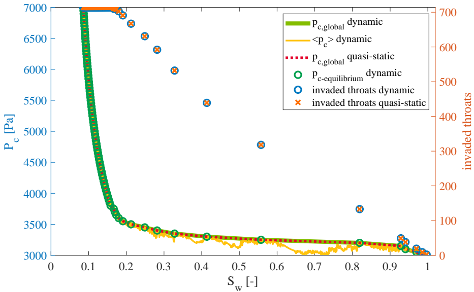
Figure 5.2: Hydrogen-water dynamic simulation compared with static simulation. The left vertical axis shows the capillary pressure and in the right vertical axis number of invaded throats is shown.
