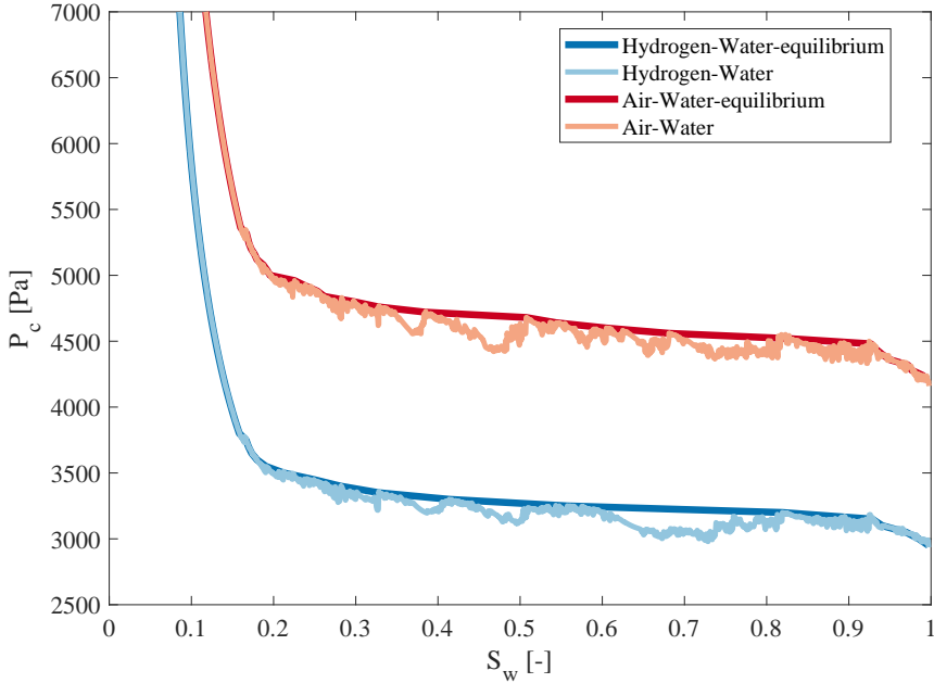
Figure 5.3: Capillary pressure function of hydrogen/water against air-water.
