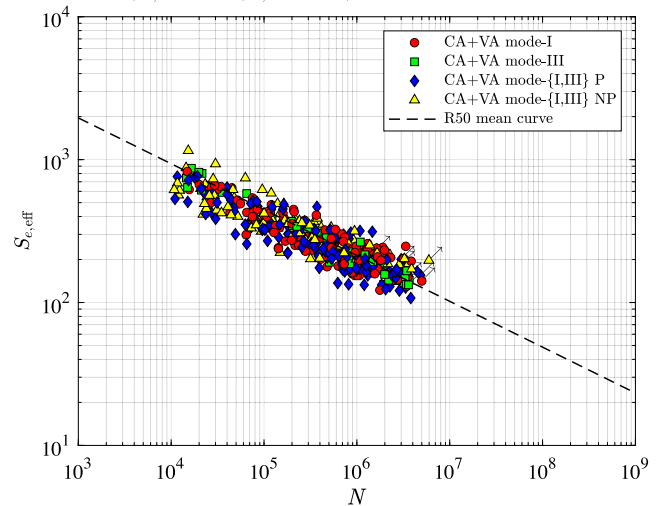
Fig. 18. Effective notch stress based fatigue resistance for uniaxial and multiaxial data; \rho_I^* \neq \rho_{III}^* and \beta = f(N) .
