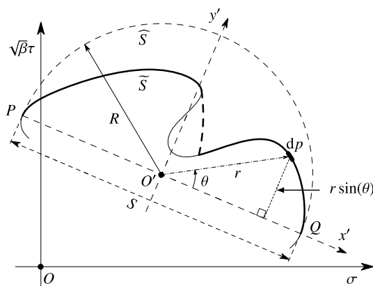
Fig. 6. Cycle-by-cycle response path based non-proportionality in the von Mises plane.
