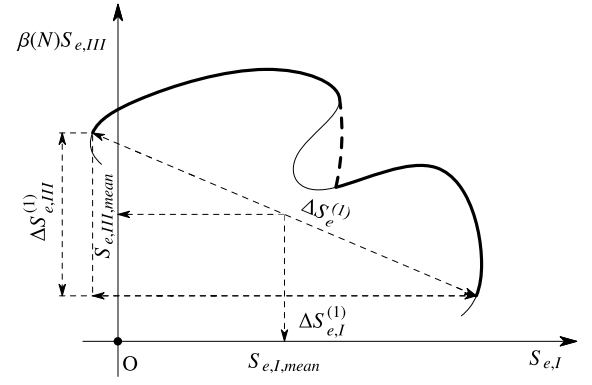
Fig. 8. Effective notch stress cycle characteristics in the von Mises plane.
