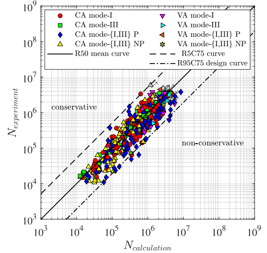
Fig. 22. Lifetime ratio plot of effective notch stress based fatigue resistance for uniaxial and multiaxial data; \rho_I^* \neq \rho_{III}^* , \beta(N) , 1st order path dependent non-proportionality with c_m = 0.65 .
