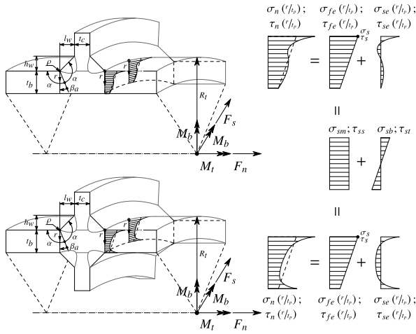
Fig. 7. Linear superposition of an equilibrium equivalent and self-equilibrium part for the mode-I, III weld toe notch shear stress distribution of a DS welded T-joint and DS welded cruciform joint in a tubular structure.
