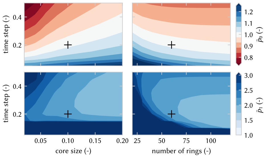
Figure 2.10: Variation of power for 2D FVW normalised by power estimate from momentum theory, for upstream (top) and downstream (bottom) turbine in a configuration as in Figure 2.1. The cross indicates the parameter choice used in this chapter. The base settings for this parameter sweep are: axial induction a_0 = 0.3 and a_1 = 0.33 , number of rings n_r = 60 , time step h = 0.2 , and core size \sigma = 0.1 .
