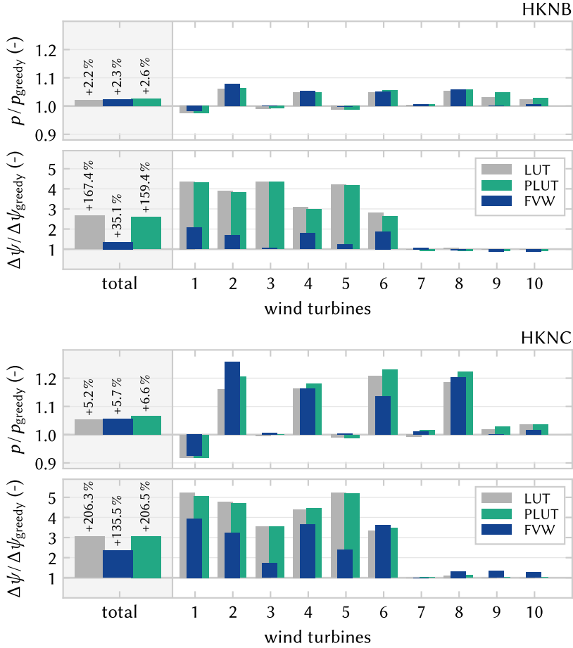
Figure 4.16: Controller performance relative to greedy control in terms of power production. In both cases, the PLUT controller yields the biggest increase in power production compared to greedy control, although the FVW controller also outperforms the LUT approach. Additionally, the FVW achieves these gains with a lower total cost in terms of yaw actuator duty. The FVW controller shows a tendency to underperform compared to the LUT for turbines 9, and 10 which are more than 12D away from their upstream neighbours for most of the simulated wind directions.
