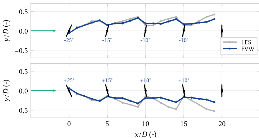
Figure 4.2: Deflection of the wake centre comparing the FVW modelling of induced yaw effects with time-averaged flow from LES. The individual FVW wakes have been combined for this comparison using a root-sum-square superposition of the wake deficit. The cumulative effect of wake steering is captured as a reduced yaw offset is required for similar levels of wake deflection when operating in the wake of yaw-misaligned turbines. The model is symmetric, whereas the LES data shows greater wake deflection from the second turbine onwards when implementing positive yaw misalignments.
