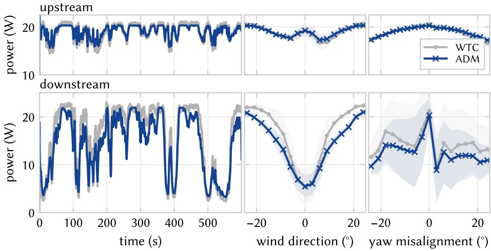
Figure 3.12: Power predictions with the ADM are compared with experimental data from WTC for the BW30 control setting. The time series fit VAF is 92.1 % for the upstream turbine and 93.3 % for the downstream turbine. The power curves for wind direction and yaw misalignment show the mean and standard deviation in 3^\circ bins. The power variation of the upstream turbine is completely due to variation in yaw misalignment from the open-loop yaw controller. The downstream power is affected both by yaw control on the upstream turbine and by translation for modelling wind direction variation. For larger wind direction magnitudes, the downstream turbine is no longer in waked conditions. The downstream effects of yaw misalignment are clouded by the variation in wind direction and therefore the power-yaw curves filtered for alignment with the wind direction are presented in Figure 3.13.
