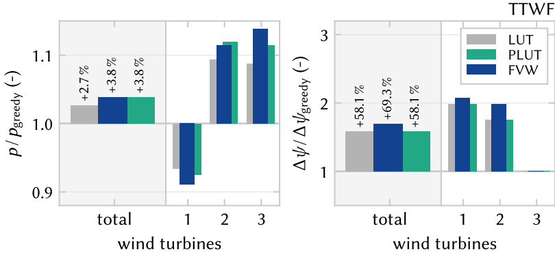
Figure 4.11: Cumulative results for the three-turbine test case in terms of total relative power production and yaw travel. The FVW controller improved power production at a slight increase in yaw travel compared to the LUT controller. In this case, the PLUT achieves the same improvement in power production as the FVW.
