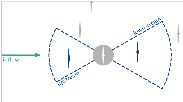
Figure 4.3: Selection of up- and downstream neighbours based on arc sectors around the inflow wind direction. The resulting directed graph connects the wind turbine in the farm in the direction of flow.
