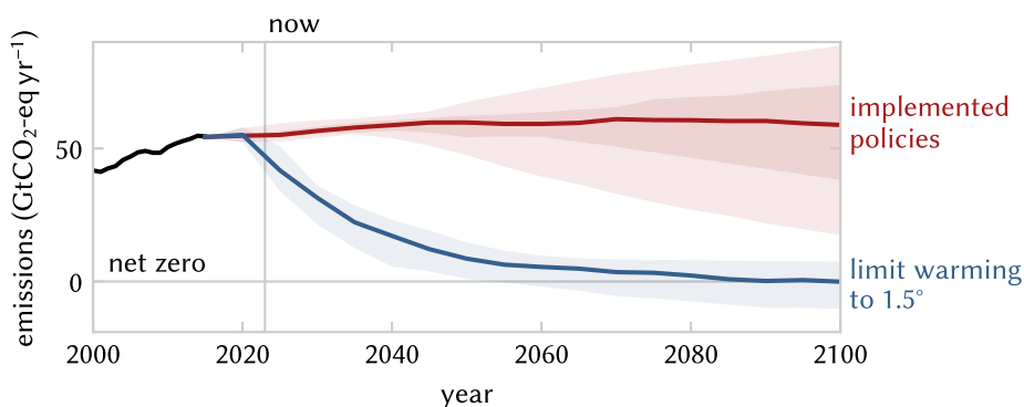
Figure 1.1: CO 2 -equivalent global emissions of greenhouse gases as presented by the IPCC [1], comparing modelled pathways that limit warming to 1.5^{\circ}\text{C} with limited or no overshoot to the modelled trajectories assuming policies implemented by the end of 2020. Major reductions in net emissions are required to reach the targets for limiting the rise of global average temperature to 1.5^{\circ}\text{C} . Data from [2].
