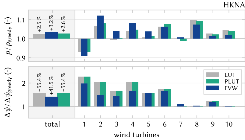
Figure 4.13: The FVW controller improves power production with respect to the LUT and PLUT approach and reduces the increase in total yaw actuation required. The gain comes mostly from turbines 2 to 7, whereas turbines 1 and 8 to 10 lose some power with respect to the LUT and PLUT controllers.
