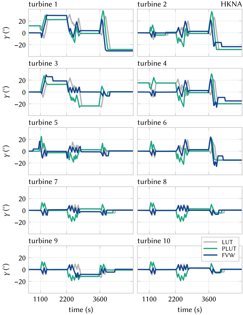
Figure 4.14: Realised yaw offsets for LUT and FVW controllers for the HKNA test case. Notably, there are some steady-state segments where turbines 1, 3, and 4 are not misaligned by the FVW controller where the LUT does prescribe a yaw offset. This is due to the limitations of the simulated wake length and prediction horizon in the current settings of the FVW controller.
