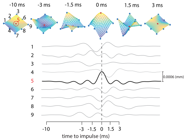
Fig. 5. Example of measured wave propagation using the inverse filter with multi actuators when focusing at the location 5. The top row shows the deformation at fixed instants. The bottom graph shows the time evolution of the displacement of all points. The deformation of point 5 is close to the Ricker wavelet used as input.
