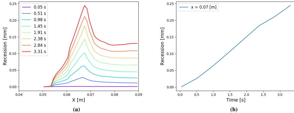
Fig. 14 Streamwise distribution of maximum (in span) recession on the compression ramp for several instances in time (a) and temporal evolution of said maximum for x = 0.07 \text{ m} .
