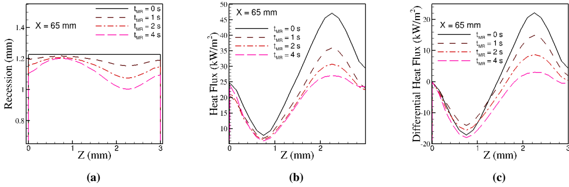
Fig. 13 Spanwise distribution at x = 0.065 \text{ m} of recession (a), heat flux (b), and differential heat flux (c) for four instances in time.
