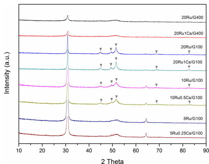
Figure 2. XRD pattern after reduction in H_2 at 673 K for Ru and Ru-Cs catalysts. (▼) Reflections from Ru(0) phase.
