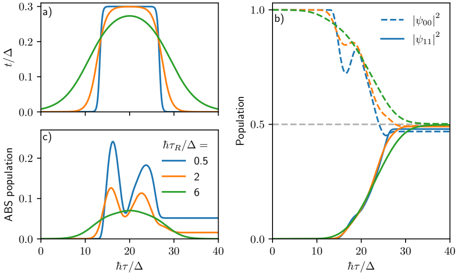
Figure 4.3: Time-dependent simulation of pairing gate \mathcal{U}_3 acting on an initial vacuum state with different pulse rise time \tau_R profiles. The vacuum population is |\psi_{00}\rangle^2 whereas the double occupation population (with middle dot unoccupied) is |\psi_{11}\rangle^2 . Longer pulses (a) result in a smoother transient population profile (b) and less leakage into the middle ABS state (c). The configuration is the spin-antiparallel with finite Zeeman field within the middle dot B/\Delta = 0.2 and symmetric spin-orbit precession \theta_L = \theta_R = \pi/8
