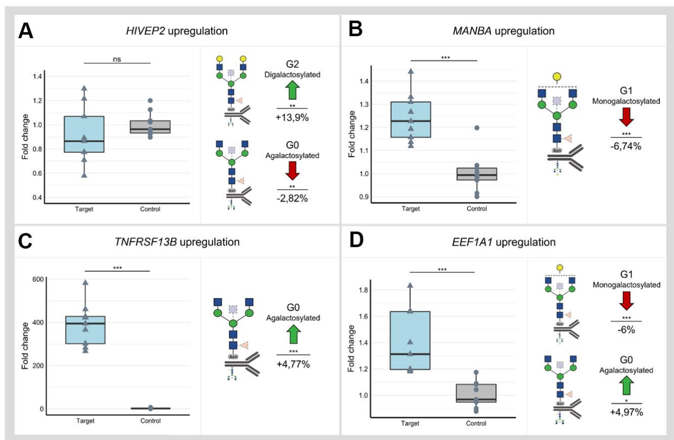
Figure 2. Changes in IgG glycan composition upon targeting of selected GWAS loci associated with IgG galactosylation ( HIVEP2 , MANBA , TNFRSF13B and EEF1A1 ) in dCas9-VPR monoclonal cell lines. Samples containing non-targeting gRNAs served as controls. Changes in transcript levels are given as fold change values and changes in IgG phenotype are given as a relative change compared to control samples. (A) Manipulation of the HIVEP2 gene did not result in a statistically significant change in HIVEP2 transcript level, however, did induce a significant increase of digalactosylated structures (G2) with a concomitant decrease of agalactosylated IgG glycan structures (G0). (B) Targeting of MANBA by dCas9-VPR elevated transcription level of this gene which resulted in decrease of monogalactosylated IgG glycan structures (G1) (C) Targeting TNFRSF13B by dCas9-VPR resulted in ~ 400-fold increase of transcript levels and significant change of IgG agalactosylated IgG glycans (G0). (D) Successful upregulation of the EEF1A1 locus was followed by an increase of agalactosylated IgG glycans (G0) with a concomitant decrease of monogalactosylated IgG glycans (G1). Nominal p-value: * <0.05 ; ** <0.01 ; *** <0.001 ; ns, not significant.
