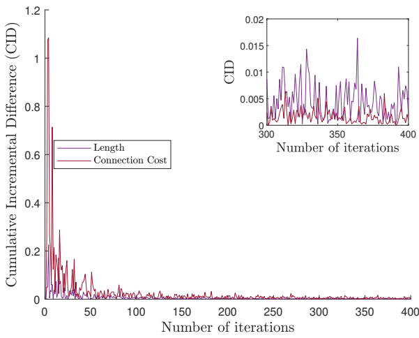
Figure 2: Convergence of the Monte Carlo simulation
