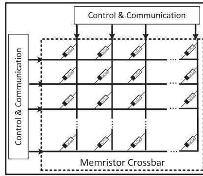
Fig. 4. The Computation-In-Memory Architecture (CIM) [51].
