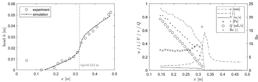
(a) Head profile in critical conditions. (b) Modeled pipe flow variables in critical conditions.
