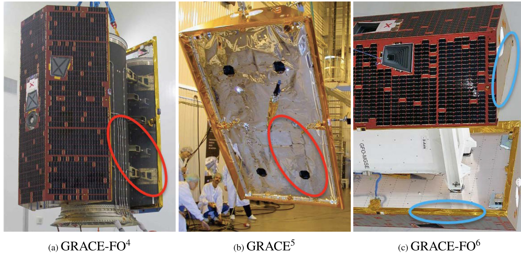
Fig. 9. Prelaunch photos of GRACE-FO 4 , 6 and GRACE 5 satellites. Red circles (a) and (b) show the differences in the nadir panel design between two satellites. Blue circles (c) indicate the differences in the material of the apron and the rear panel.
