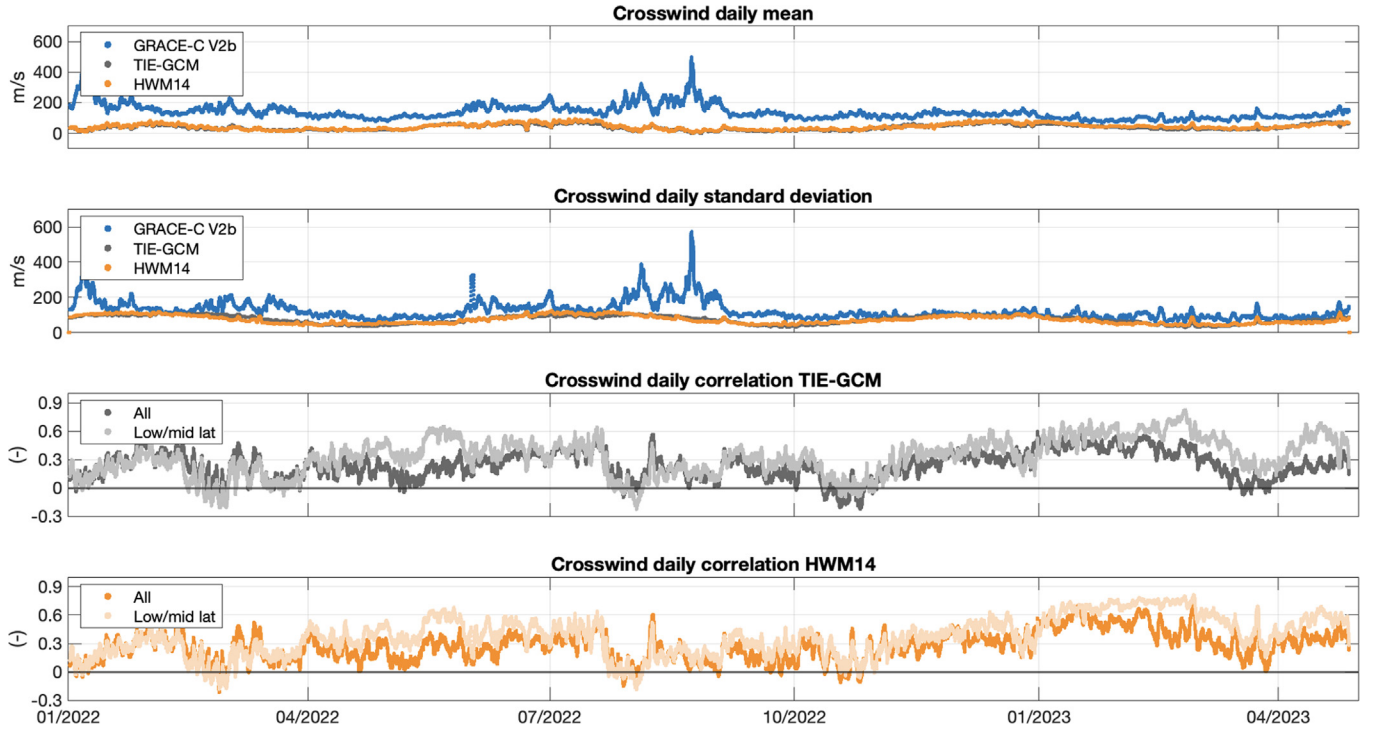
Fig. 15. Statistical comparison of the crosswind speed observed by the GRACE-C and model estimates from HWM14 and TIE-GCM. Two top panels show the daily mean and the daily standard deviation. Two bottom panels show the Pearson's correlation coefficient for TIE-GCM and HWM14, respectively, for two types of subsets: all data and low- to mid-latitudes. The values on the x-axis are common for all plots.
