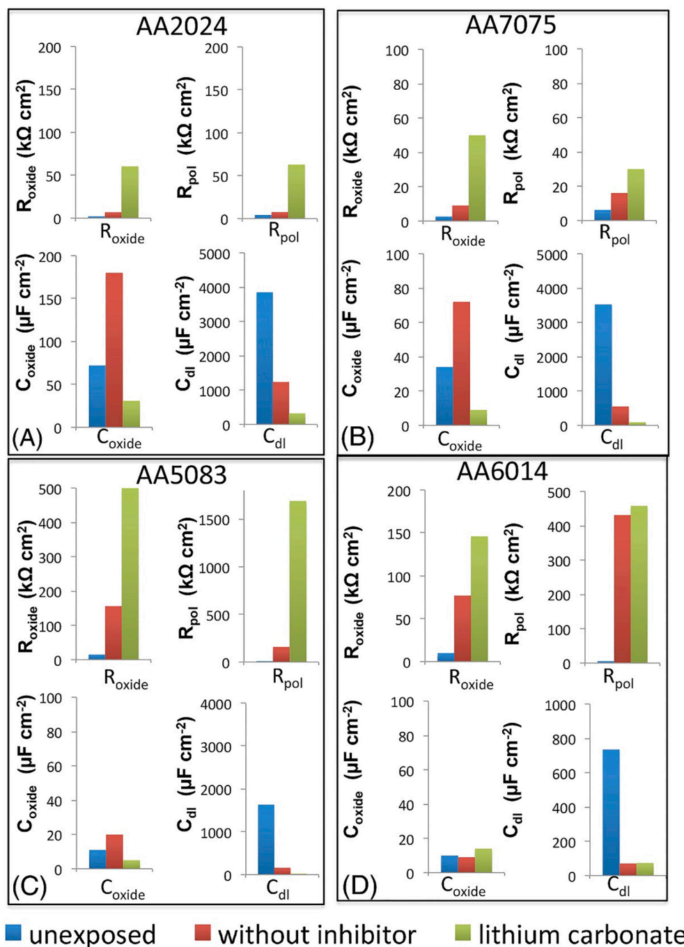
Fig. 8. Results of the electrochemical parameters including oxide resistance ( R_{\text{oxide}} ), polarization resistance ( R_{\text{pol}} ), oxide capacitance ( C_{\text{oxide}} ), and double layer capacitance ( C_{\text{dl}} ) inside the artificial defects of different aluminium alloys covered by coatings loaded with and without \text{Li}_2\text{CO}_3 before and after neutral salt spray test: A, AA2024; B, AA7075; C, AA5083; and D, AA6014 [111].
