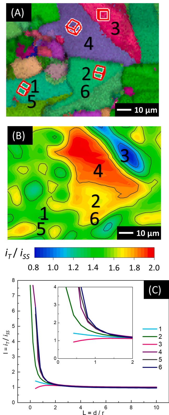
Fig. 6. (A) EBSD orientation map and (B) SECM map ( 100 \times 80 \mu\text{m}^2 ) of the polished growth surface (same area) obtained with a 10 \mu\text{m} diameter Pt tip in 1 mM \text{FcMeOH}^{+/0} (in 0.1 M \text{KNO}_3 ), with a tip potential of +0.5 V (vs. \text{Ag}/\text{AgCl} ) and the BDD substrate kept under OCP. (C) Experimental probe approach curves recorded at the six different spots, as indicated by the numbers in (A) and (B).
