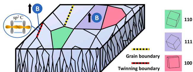
Fig. 7. Schematic representation of the investigated features on the free-standing, polycrystalline BDD electrode.
