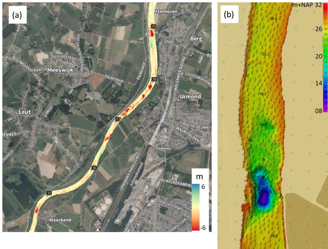
Figure 11: Bed level changes Common Meuse (a) between Maasband (rkm 34) and Nattenhoven (rkm 39.5) and (b) detail of scour hole near the ferry crossing of Berg (source: RWS CIV). Purple colours in figure b indicate low bed levels and red high. Water is flowing from the bottom to the top of the map.
