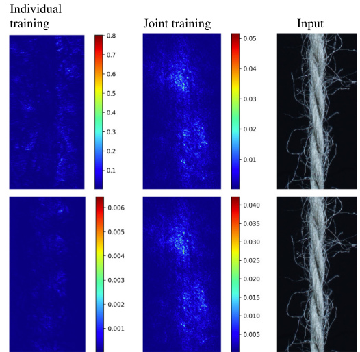
Fig. 7. Saliency maps for the yarn twist pitch \alpha_{pty} (top row) and the yarn radius R_{pty} (bottom row), obtained from the individual training of Reg for each parameter (left) vs. the joint training of Reg (middle).
