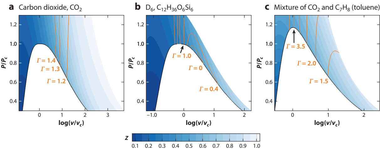
Figure 2 Exemplary isolines of the fundamental derivative of gas dynamics in the pressure-volume thermodynamic plane (reduced variables), where P is pressure, P_c is critical pressure, v is volume per unit mass, v_c is critical volume per unit mass, and \Gamma is the fundamental derivative of gas dynamics. (a) Low molecular complexity fluid. (b) Bethe-Zel'dovich-Thompson fluid. (c) Equimolar mixture that is a high molecular complexity fluid.
