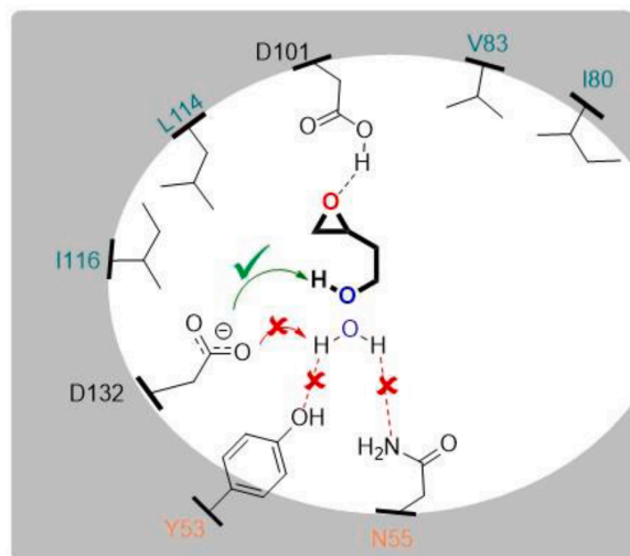
Fig. 10. Epoxide hydrolase engineered to catalyze a Baldwin-type cyclisation.
