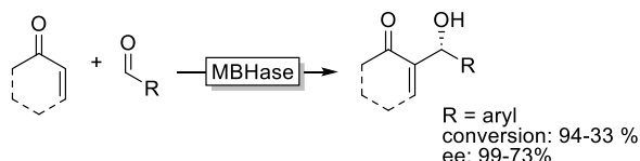
Fig. 9. Newly designed enzyme to catalyze Morita-Baylis-Hillman reactions.
