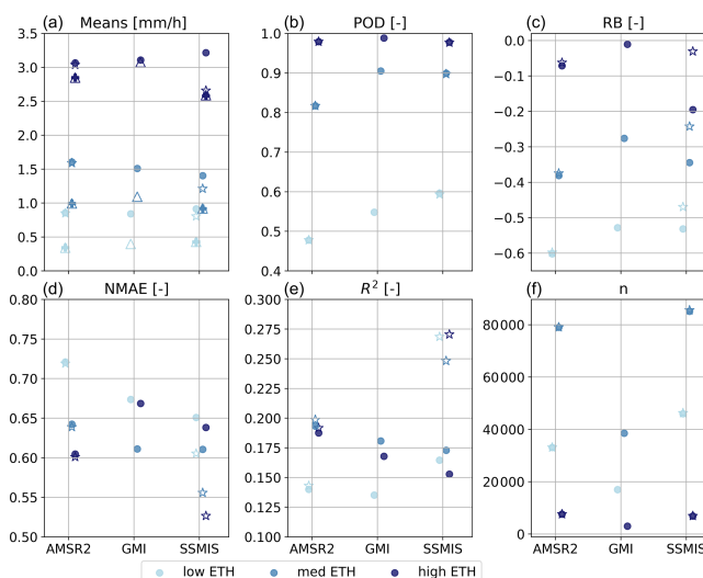
Figure 2. Statistics of GPROF for the three sensors using reference estimates averaged over the footprint associated with the GMI 19 GHz channel (circles) or each sensor's own 19 GHz channel (stars). The triangles (GMI 19 GHz channel) and pluses (own sensors 19 GHz channel) in (a) represent GPROF's mean. Additionally, the vertical extent of precipitation was taken into account (different blue shades). The statistics are based on all overpasses during the study period. Except for the contingency metric (POD), paired observations where both references exceed 0.1 \text{ mm h}^{-1} (hits) and 1 \text{ km} \leq \text{ETH} < 15 \text{ km} are considered.
