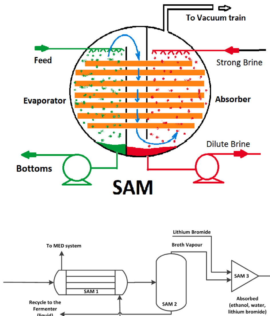
Fig. 7. Stripping-absorption module (SAM) working principle and the corresponding equivalent of conventional units (usable in Aspen Plus simulations).
