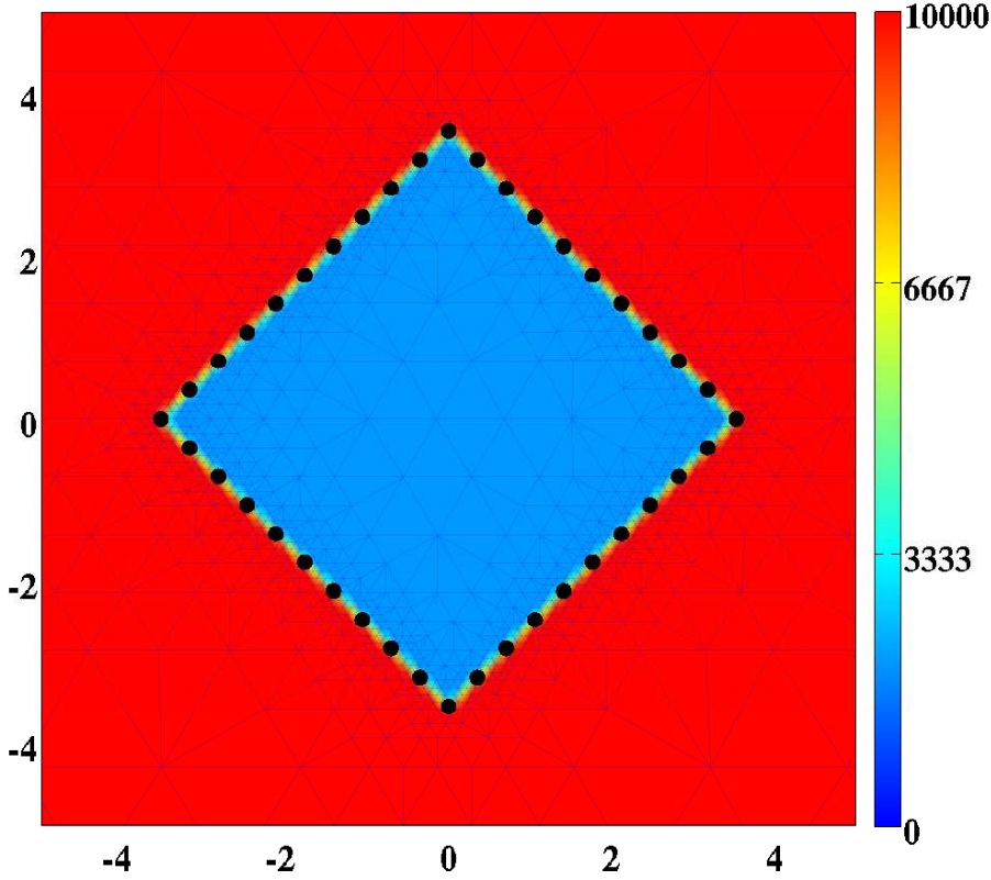
Figure 7.1: A graphical overview of the initial conditions. Depicted are the initial shape of the skin graft and, in color scale, the initial cell density of the fibroblasts (cells/cm 3 ). The scale along both axes is in centimeters. The X -axis points toward the reader. The black dots mark the material points that were used to trace the evolution of the surface area of the skin graft over time. That is, at each time point, the area of the polygon with vertices located at the displaced black material points was determined
