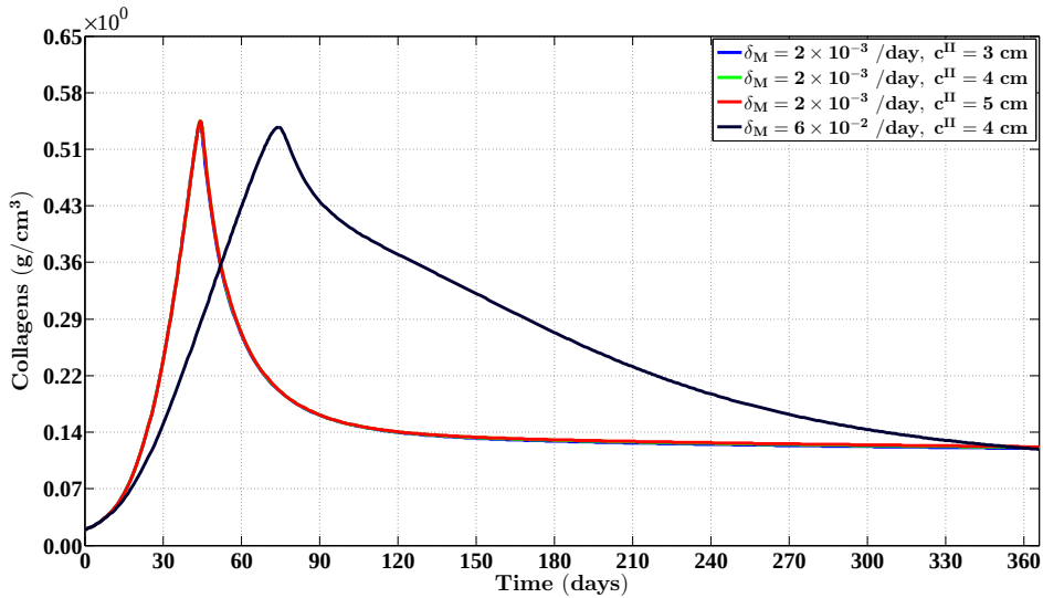
Figure 6.7: The evolution over time of the concentration of the collagen molecules for different values for the apoptosis rate of myofibroblasts and various widths of the wound (The blue curve and the green curve are situated underneath the red curve). All other parameter values are equal to those depicted in Table 6.1. See Subfigure 6.1c for the location where the evolution of the concentration was traced over time
