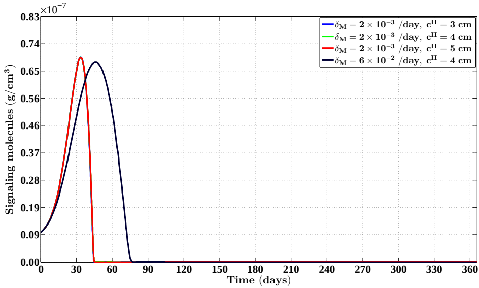
Figure 6.6: The evolution over time of the concentration of the signaling molecules for different values for the apoptosis rate of myofibroblasts and various widths of the wound (The blue curve and the green curve are situated underneath the red curve). All other parameter values are equal to those depicted in Table 6.1. See Subfigure 6.1c for the location where the evolution of the concentration was traced over time
