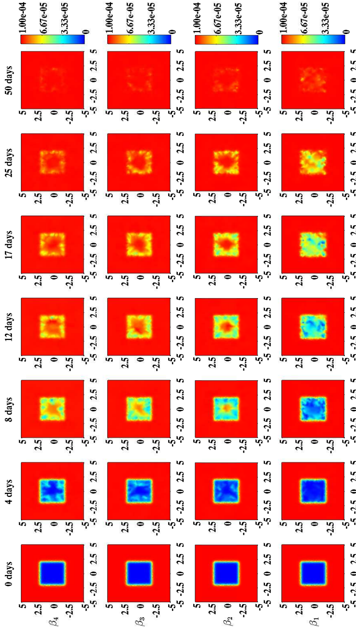
Figure 3.8: An overview of the evolution over time of the concentration of the collagen molecules for the constant \beta_M \phi related to the number of monocytes that transigrate per time step. Here \beta_1 = 0.00 \times 10^{10} \text{ mm}^2/(\text{g h}) , \beta_2 = 2.50 \times 10^{10} \text{ mm}^2/(\text{g h}) , \beta_3 = 5.00 \times 10^{10} \text{ mm}^2/(\text{g h}) and \beta_4 = 7.50 \times 10^{10} \text{ mm}^2/(\text{g h}) . In these simulations the value for the receptor binding rate of the TGF- \beta molecules is 5 \times 10^{11} \text{ mm}^3/(\text{g h}) . The values for the other parameters are equal to those depicted in Table 3.1. The color scales represent the concentrations, measured in \text{g}/\text{mm}^3 . Within the subfigures, the scale along both axes is in millimeters
