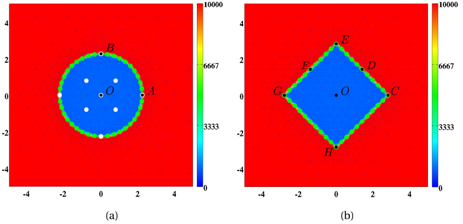
Figure 4.1: Graphical representations of the initial conditions. Depicted are in both subfigures, the initial shape of the wound and, in color scale, the initial cell density of the fibroblasts (cells/cm 3 ). In both subfigures the scale along both axes is in centimeters. In Subfigure 4.1a, the white dots mark the material points where the evolution of the cell density / concentration of the different modeled constituents was traced over time for the generation of some of the figures in Section 4.4. In both subfigures, the green dots mark the material points that were used to trace the evolution over time of the surface area of the wound. That is, at each time point the area of the polygon with vertices located at the displaced green material points has been determined. Finally, the material points labeled with a letter have been used to study the evolution over time of the shape of the wound. See Section 4.4 for more details on this matter
