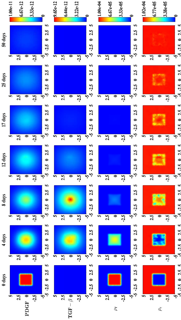
Figure 3.2: An overview of simulation results for continuous primary variables of the model when the value for the constant \beta_{M\Phi} is 7.50 \times 10^{10} \text{ mm}^2/(\text{g h}) and the value for the receptor binding rate of the TGF- \beta molecules is 5 \times 10^{11} \text{ mm}^3/(\text{g h}) . The values for the other parameters are equal to those depicted in Table 3.1. From top to bottom, the rows show the evolution over time of the concentration of, respectively, the PDGF molecules, the TGF- \beta molecules, the fibrin molecules and the collagen molecules. The color scales represent the concentrations, measured in \text{g/mm}^3 . Within the subfigures, the scale along both axes is in millimeters
