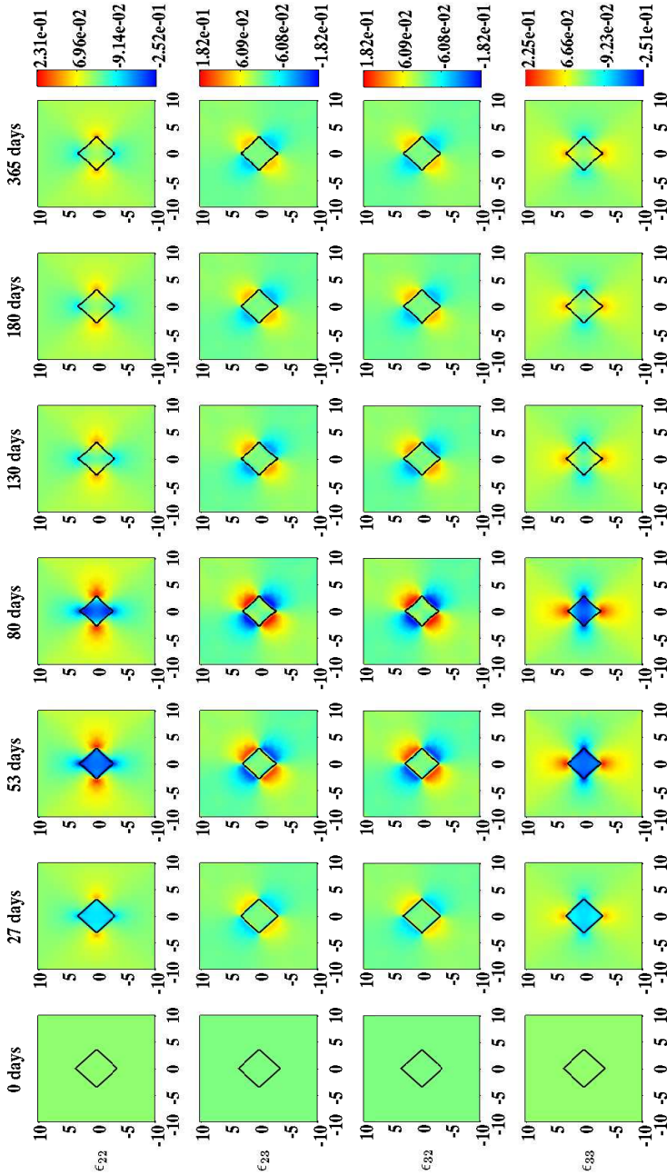
Figure 7.4: An overview of simulation results for the effective strain when the inhibition of the secretion of MMPs due to the presence of signaling molecules is relatively low ( \zeta_c^{III} = 2 \times 10^8 \text{ cm}^3/\text{g} ) and the rate of morphoelastic change is relatively high ( \zeta = 9 \times 10^2 \text{ cm}^6/(\text{cells g day}) ). The values for all other parameters are equal to those depicted in Table 7.1. The separate rows show the evolution over time of the different components of the effective strain that are unequal to zero. The color scales represent the amount of effective strain. Within the subfigures, the scale along both axes is in centimeters. The black squares within the subfigures represent the (displaced) boundaries between the skin graft and the unwounded dermis
