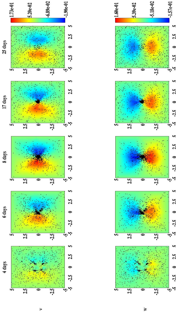
Figure 3.5: An overview of simulation results for the demonstration of the relationship between the position of the cell centers of the fibroblasts and the nonzero components of the displacement field. In this simulation the value for the constant \beta_{M\Phi} is 7.50 \times 10^{10} \text{ mm}^2/(\text{g h}) and the value for the receptor binding rate of the TGF- \beta molecules is 5 \times 10^{11} \text{ mm}^3/(\text{g h}) . The values for the other parameters are equal to those depicted in Table 3.1. The rows show the evolution over time of the displacement in, respectively, the horizontal direction and the vertical direction. The color scales represent the displacement, measured in mm. The black circles mark the positions of the cell centers of the fibroblasts. Within the subfigures, the scale along both axes is in millimeters
