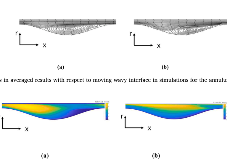
Fig. 8. Turbulent kinetic energy k^+ with respect to moving wavy interface in simulations for the annulus; (a) RANS, (b) DNS. (lower values in blue, and higher values in yellow).
