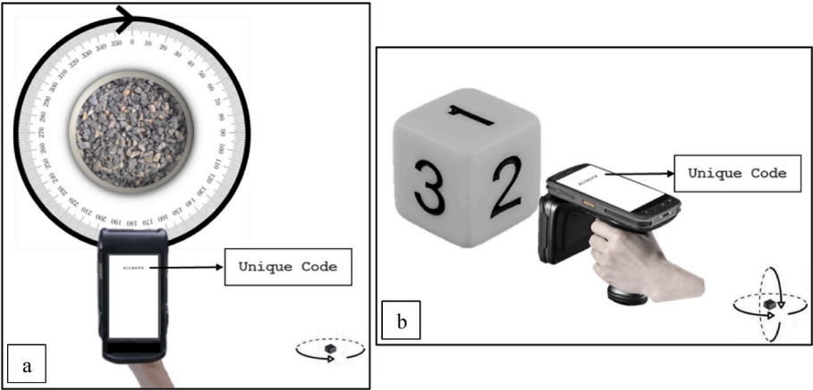
Fig. 4. a) The method of assessing the readability performance of RFID tags embedded in concrete components; b) The method of labeling and assessing the readability performance of RFID tags embedded in cube-shaped concrete samples.
