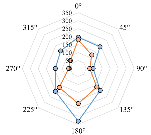
Fig. 13. Average readability of RFID tag types CS, CM, and CL in cm in concrete beam.
