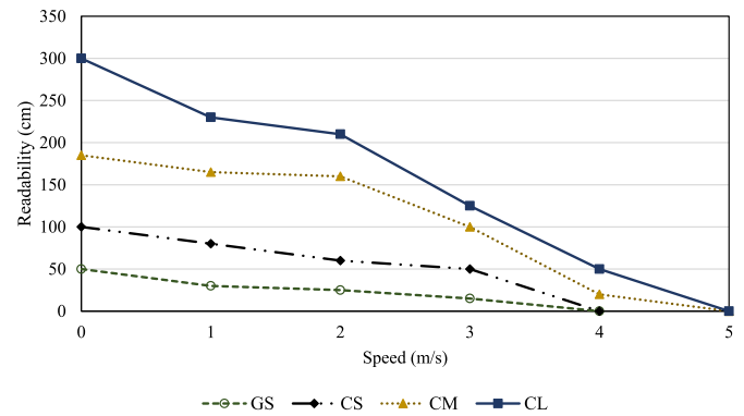
Fig. 9. The RFID tags responses at different speeds.
