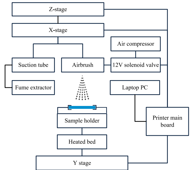
Fig. 2. The principle construction of the spray printer.
