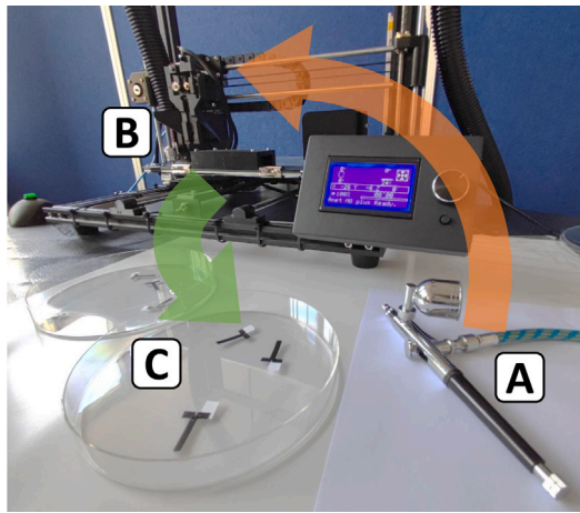
Fig. 1. The proposed concept: introducing an airbrush tool (A) into a 3D printer (B) for spray printing smart material transducers (C).
