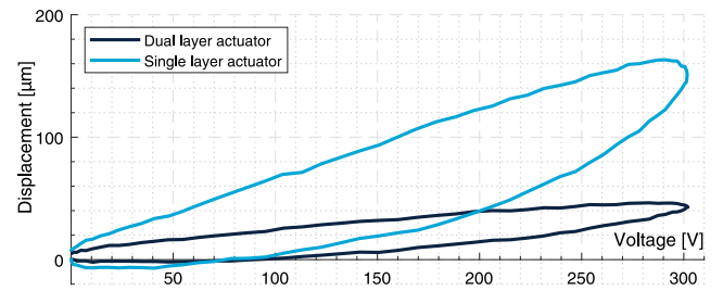
Fig. 19. Actuation hysteresis upon unipolar excitation (1 Hz).
