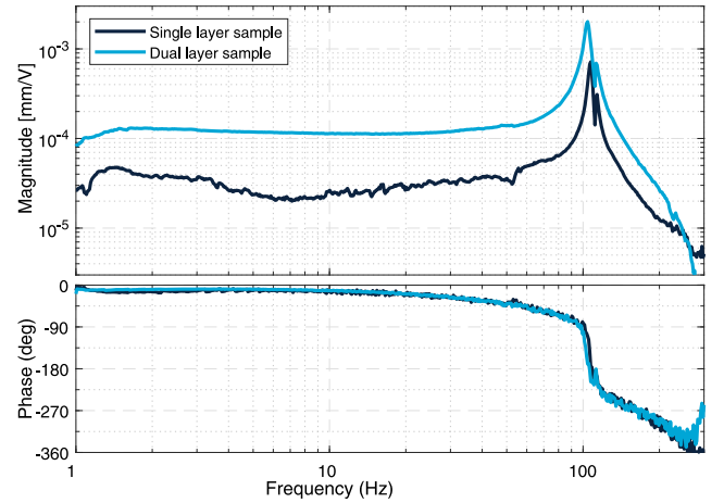
Fig. 18. Frequency responses of the single- and dual-layer actuators upon 100 V_{pp} excitation.
