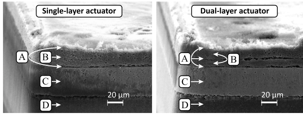
Fig. 15. SEM images of the actuator cross-sections. The visible components are indicated as: A – the electrodes; B – the EAP layers; C – the microporous resin portion of the substrate; and D – the PET substrate.
