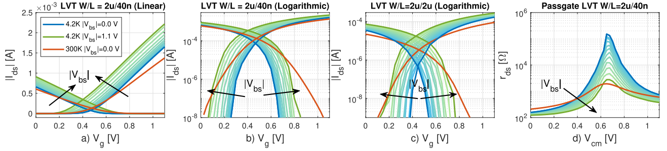
Fig. 1. DC measurements of LVT NMOS/PMOS devices at 300 K (red line) and 4.2 K (green to blue lines). For the 4.2-K results, the body-biasing |V_{bs}| is swept from 0 V to 1.1 V in steps of 0.1 V (shades). To improve readability, the leakage is subtracted. The NMOS source is grounded, and the PMOS source is connected to V_{dd} = 1.1 V. (a-b) I_{ds}/V_g at |V_{ds}| = 1.1 V for W/L = 2\mu\text{m}/40\text{nm} in linear and semi-logarithmic scale. (c) W/L = 2\mu\text{m}/2\mu\text{m} in semi-logarithmic scale. (d) Small-signal resistance of the pass gate vs. the voltage applied on the drain/source, obtained by numerically combining in parallel the individually measured NMOS and PMOS resistance of (a-b).
