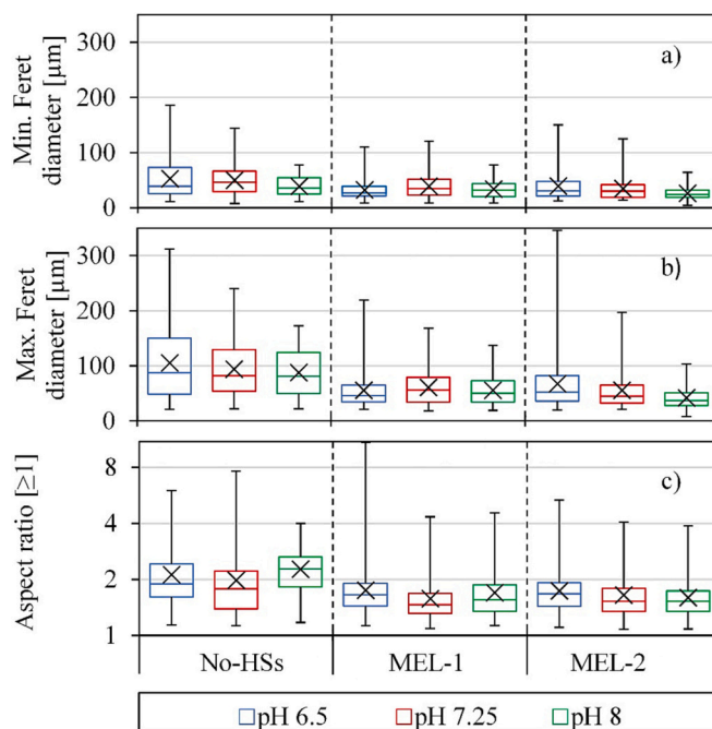
Fig. 3. PSD analysis of the crystallisation experiments: a) Minimum Feret diameter; b) Maximum Feret diameter; c) Aspect ratio (logarithmic scale). HSs data are not shown, since precipitates could not be determined.
