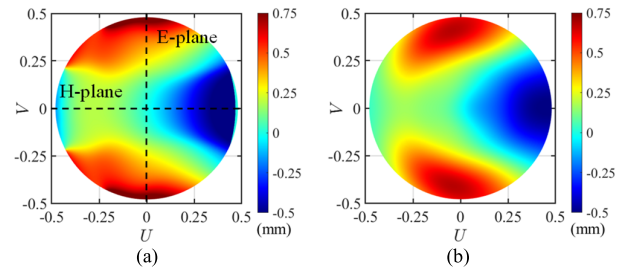
Fig. 10. Optimized lens surface modification: (a) ideal one and (b) smoothed Zernike surface.
