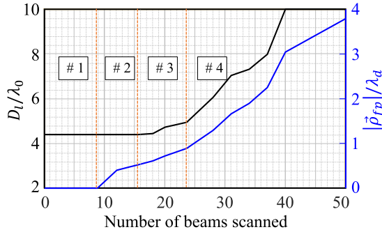
Fig. 6. Flash point \vec{p}_{fp} and lens diameter D_l versus the number of beams scanned. The orange lines show the border of the four regions of the FPA.
