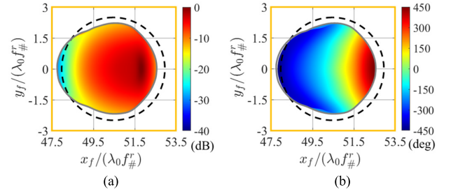
Fig. 12. Lens GO field on the lens aperture S_{ap} within the orange area depicted in Fig. 9: (a) amplitude and (b) phase.
