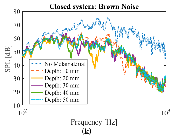
Figure 13. Noise amplitude measurements for the closed system for different isolated frequencies and white, pink and brown noise samples.
