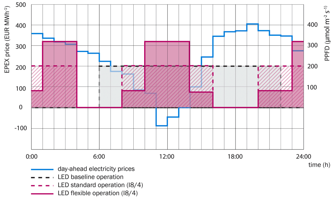
Fig. 12b. LED operation I8/4 standard versus flexible operation on July 24th, 2022.
