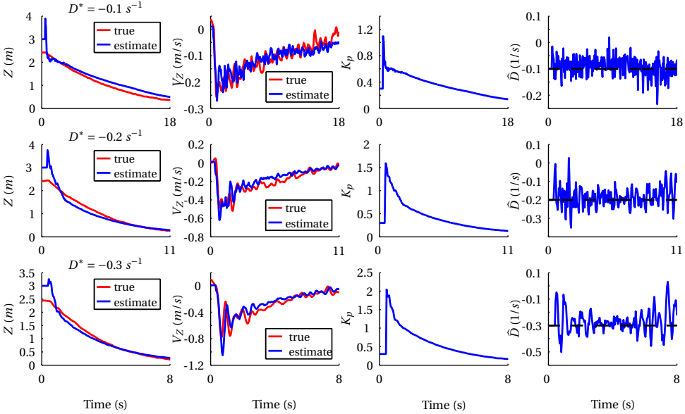
Figure 2.9: Height-adapted control for constant flow divergence landings with different flow divergence set points ( D^* = -0.1, -0.2, -0.3 \text{ s}^{-1} ).
