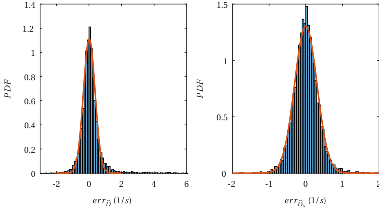
Figure 3.11: Probability density functions of the estimate errors of \hat{D} (left) and \hat{D}_s (right) with respect to the fitted model.
