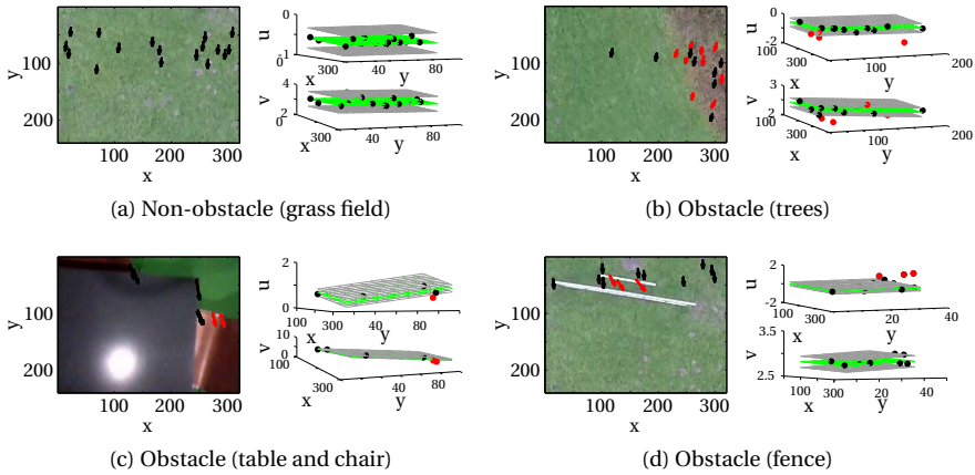
Figure 5.5: Outdoor and indoor images without and with obstacles, and their corresponding optical flow fits. Non-obstacle: Consistent optical flow vectors (black) contribute to low fitting errors. Obstacle: Irregular optical flow vectors (red) lead to high fitting errors.
