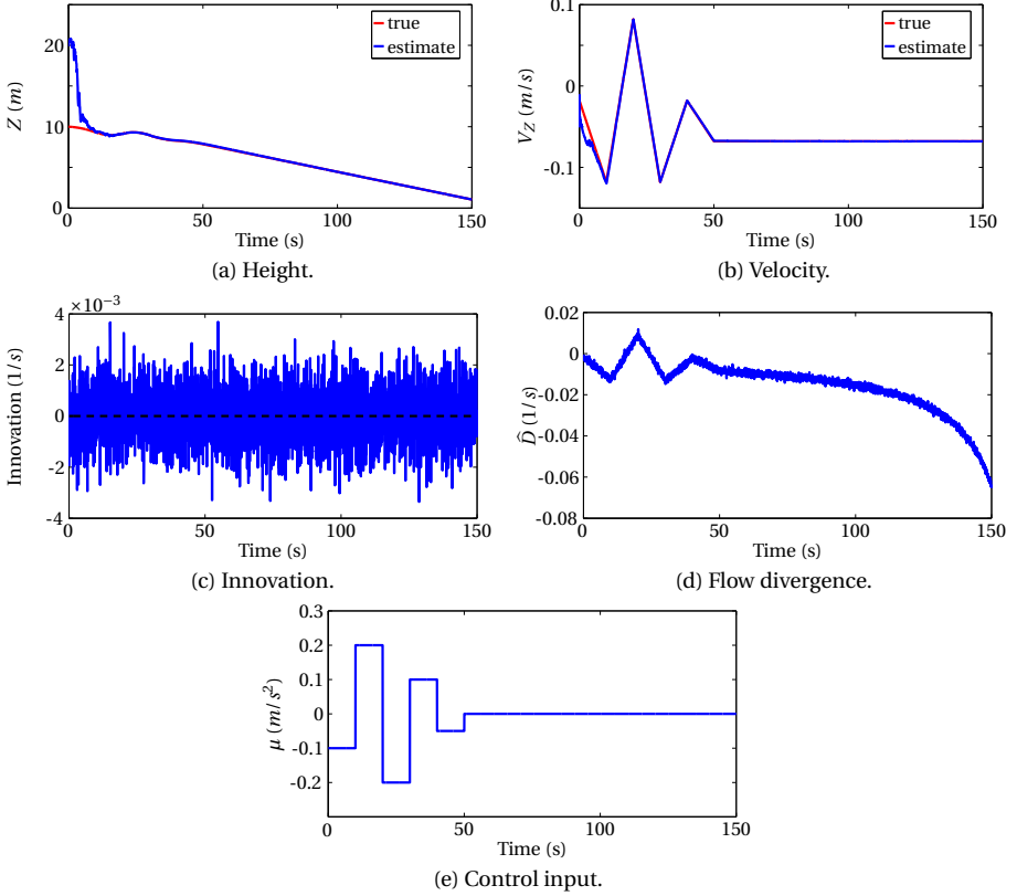
Figure 2.5: EKF-based height and vertical velocity estimation from flow divergence for landing control.
