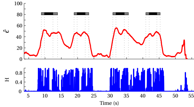
Figure 5.15: Uncertainty measure H (bottom) and roughness estimate \hat{\epsilon} (top) in E2.
