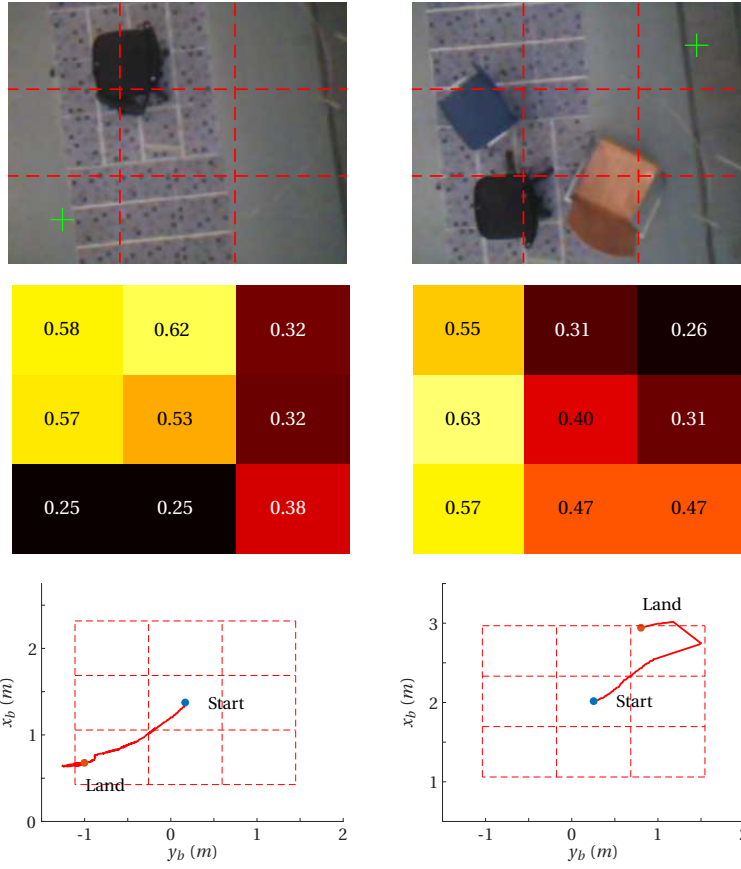
Figure 5.24: Indoor Experiment: Cross markers in the top row images show the chosen landing spot. Center row presents \hat{\epsilon} for all regions with color scaled according \hat{\epsilon} (Yellow = obstacle; Black = non-obstacle). Bottom row presents the flight path of the MAV from the time when the landing strategy activated until the time when it landed.
