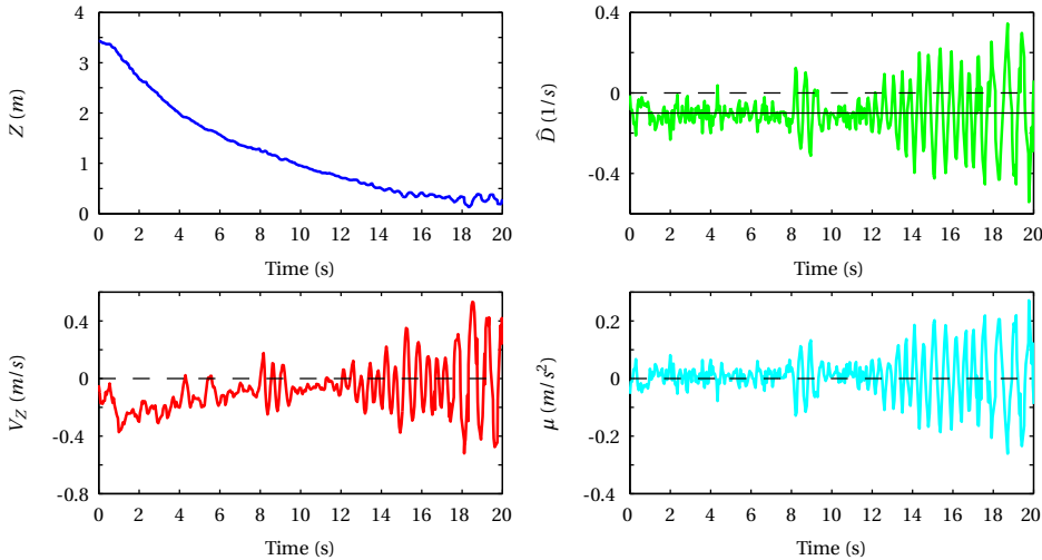
Figure 3.14: Constant flow divergence landing of the MAV using a fixed-gain controller.
