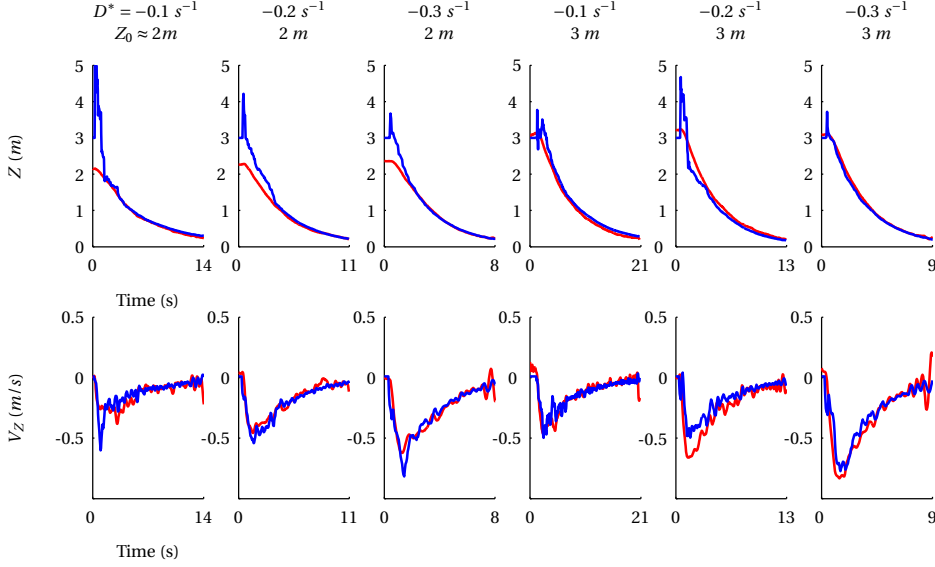
Figure 2.8: Fixed-gain multiple landings with different flow divergence set points ( D^* = -0.1 \text{ s}^{-1}, -0.2 \text{ s}^{-1}, -0.3 \text{ s}^{-1} ) at different initial heights ( Z_0 = 2\text{m}, 3\text{m} ). The estimates are shown with blue lines while their true values are represented by red lines.
