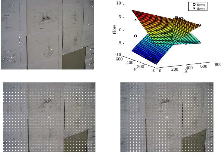
Figure 4.2: Illustration of the vision process. Top left: the determined optical flow vectors. Top right: quadratic fits for the flow in x-direction (circle markers) and y-direction (cross-markers). Bottom left: estimated flow field in x-direction. Bottom right: estimated flow field in y-direction. The motion of the camera is straight towards the wall, which has an angle of \sim 45^\circ to the camera axis.
