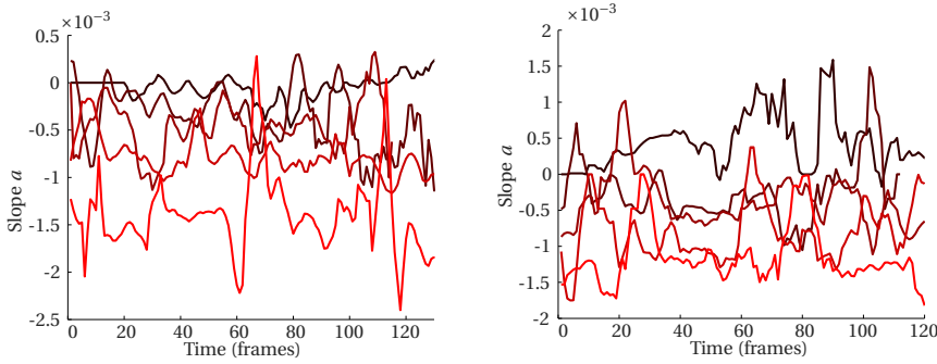
Figure 4.6: Results of slope estimation on video sequences. Left: motion in Y -direction. Right: motion in X -direction. The plots show the estimated slope a (y-axis) over time (x-axis). The brightness of the lines are determined by the angle with the wall, with the darkest color corresponding to 0 degrees and the brightest color corresponding to 60 degrees.
