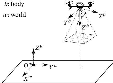
Figure 3.1: MAV body ( O^b X^b Y^b Z^b ) and world ( O^w X^w Y^w Z^w ) reference frames.
