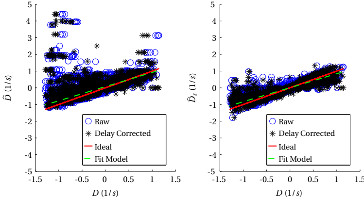
Figure 3.9: Deviation of the estimated flow divergences \hat{D} (left) and \hat{D}_s (right) from their ground truth D .
