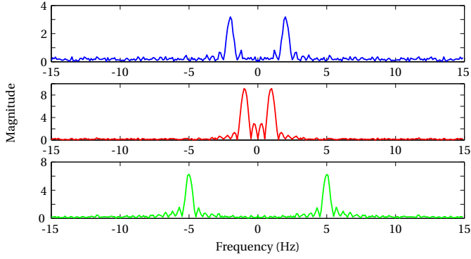
(b) Discrete Fourier Transform of the generated signals.
