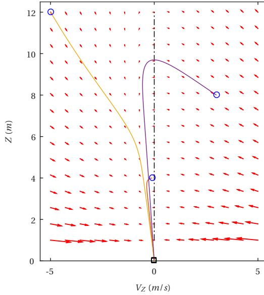
Figure 3.16: Phase portrait of the constant flow divergence landing.
