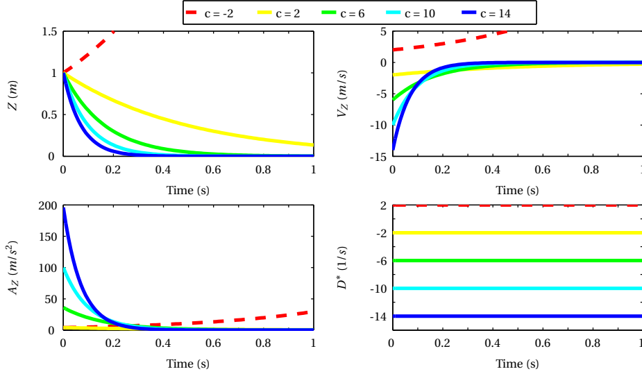
Figure 3.3: Constant flow divergence guidance with different desired flow divergence D^* = -c .
