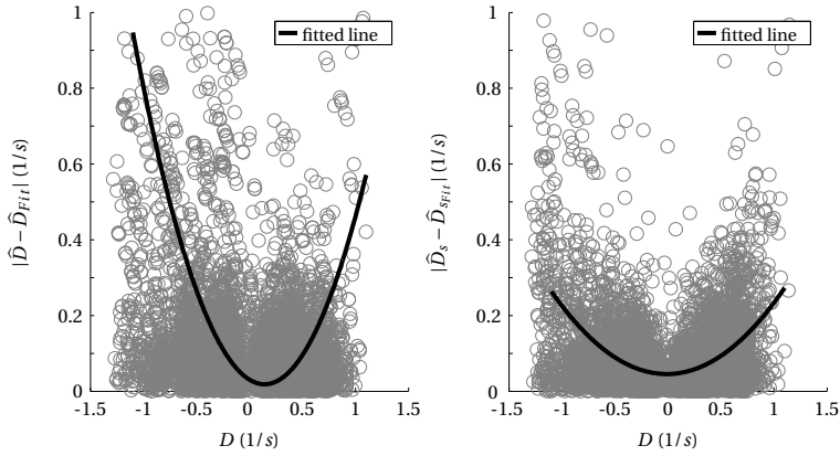
Figure 3.10: Absolute errors of the flow divergence estimates \hat{D} (left) and \hat{D}_s (right) versus their ground truth D .
