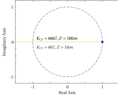
Figure 3.17: Root locus of the closed-loop discrete system for two different heights.
