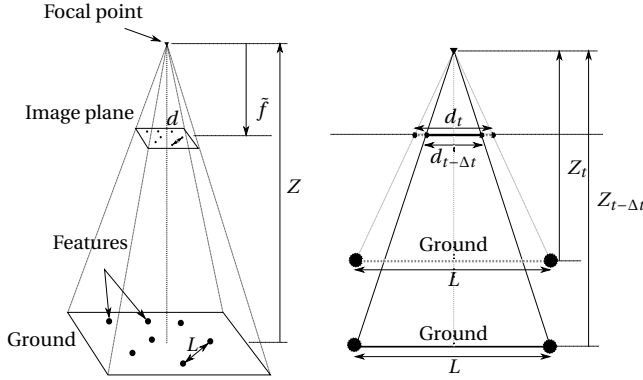
Figure 3.5: Pinhole camera model (left) and projected lines on image plane when approaching ground (right).
