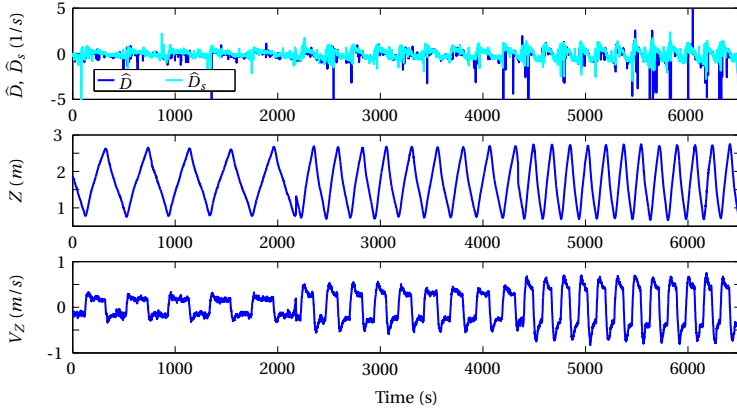
Figure 3.7: Log of flow divergence estimates, height, and vertical velocity during a vertical maneuver of an AR.Drone 2.0.
