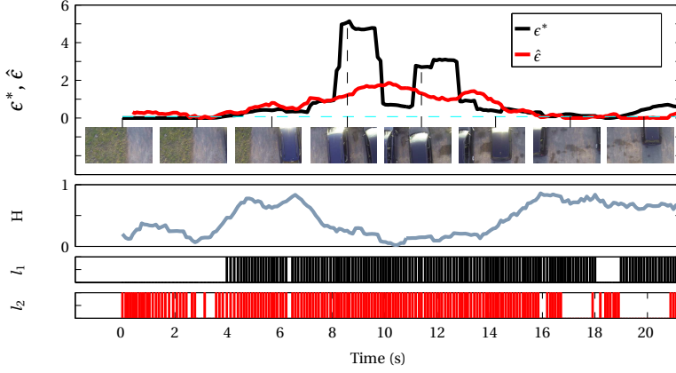
Figure 5.19: Classification of obstacles with \epsilon^* ( l_1 ) and \hat{\epsilon} ( l_2 ) in an untrained outdoor scene (S3), and the corresponding uncertainty measure, H. This example with a particular threshold of \hat{\epsilon}_{th} = 0.076 is chosen in the K-fold validation 2 which resulted in TP rate of 0.9 and FP rate of 0.5.
