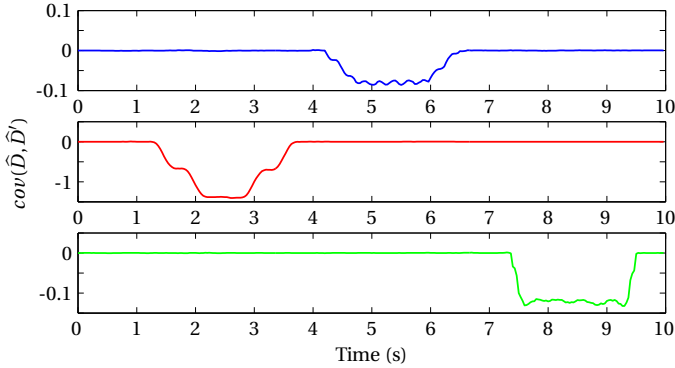
(c) Covariances of the generated signals with delays \frac{1}{2}\mathcal{P} matching the half periods of the frequencies.
