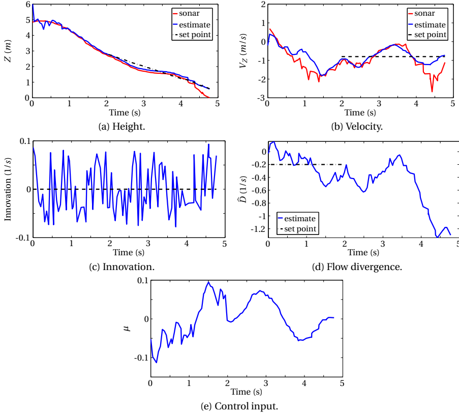
Figure 2.11: Landing with a linear controller using estimates from EKF (Outdoor Flight).
