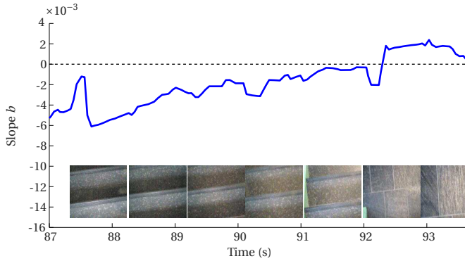
Figure 4.11: Real-time slope estimation results with the Parrot AR drone's bottom camera. The plot shows the estimated slope b and images taken from the onboard camera over time ( x -axis)
