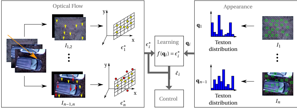
Figure 5.1: Overview of the novel self-supervised learning (SSL) setup. The MAV starts flying using a roughness measure \epsilon^* extracted from optical flow algorithm (left). A function is learned that maps appearance features, \mathbf{q} from a still image to an estimate of the roughness measure \hat{\epsilon} (right). After learning, the MAV can determine whether there are obstacles below based on a still image, allowing landing site selection in hover.
