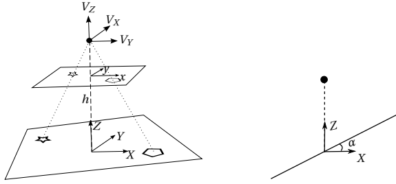
Figure 5.2: Left: A pin hole model. Right: An inclined ground surface with slope \alpha .
