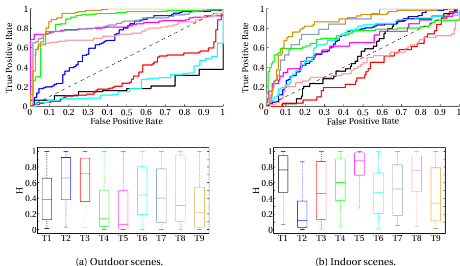
Figure 5.18: ROC curves and uncertainty measures for K-fold cross-validations 2. The results are given the color of the test scene (see Fig. 5.4).
