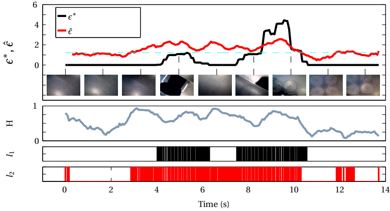
Figure 5.20: Classification of obstacles with \epsilon^* ( l_1 ) and \hat{\epsilon} ( l_2 ) in an untrained indoor scene (S3), and the corresponding uncertainty measure, H. This example with a particular threshold of \hat{\epsilon}_{th} = 1.225 is chosen in the K-fold validation 2 which resulted in TP rate of 0.9 and FP rate of 0.5.
