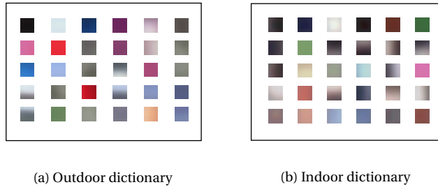
Figure 5.8: Trained dictionaries used in texton method for scene S5 in outdoor and indoor datasets.
