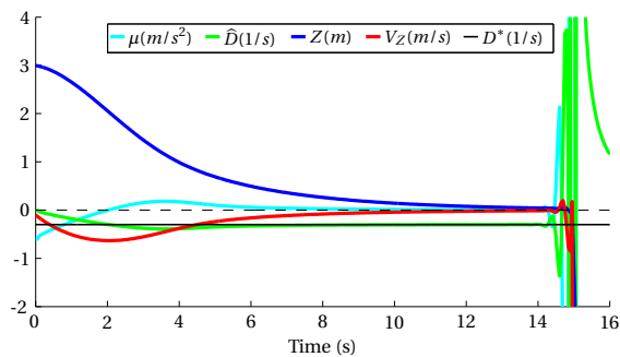
(a) Adding delay.
