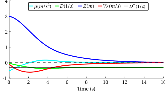
Figure 3.4: Fixed-gain closed-loop landing control using a constant flow divergence strategy.
