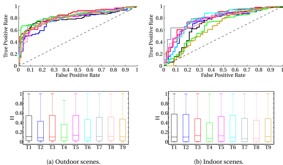
Figure 5.17: ROC curves and uncertainty measures for K-fold cross-validations 1. The results are given the color of the test set.
