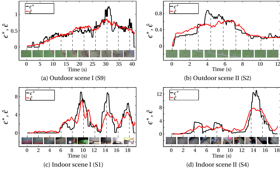
Figure 5.6: Obstacle detection using roughness estimates \epsilon^* from optical flow algorithm and \hat{\epsilon} from appearance while navigating.
