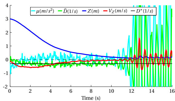
(c) Adding delay and noise model.
