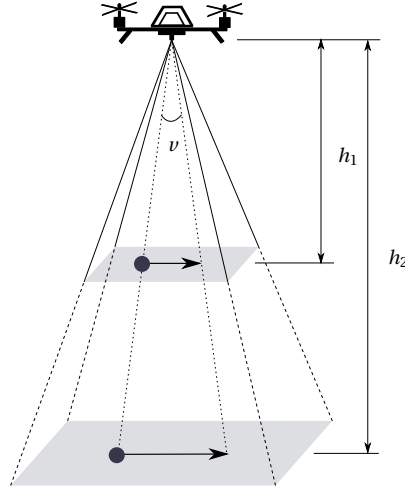
Figure 1.4: ‘Scale-less’ property of optical flow. This property can be clearly seen from the case that the same amount of optical flow v can be perceived by a stationary observer from a near, slow-moving object and a distant, fast-moving object. For instance, if v = 1 \text{ s}^{-1} , it could be perceived from an object that moves at 1 \text{ ms}^{-1} at h_1 = 1 \text{ m} or at 10 \text{ ms}^{-1} at h_2 = 10 \text{ m} .
