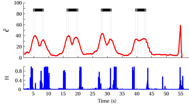
Figure 5.14: Uncertainty measure H (bottom) and roughness estimate \hat{\epsilon} (top) in E1.
