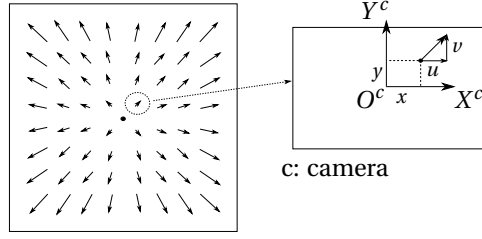
Figure 3.2: Divergence of optical flow (flow divergence) when an observer is approaching a surface.
