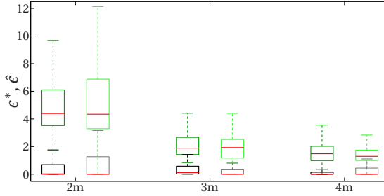
Figure 5.26: Effect of height on roughness. Dark green and light green boxplots represent the roughness \epsilon^* and \hat{\epsilon} , respectively measured in the presence of obstacles. Black and gray boxplots represent the roughness \epsilon^* and \hat{\epsilon} , respectively measured in the absence of obstacles.
