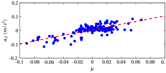
Figure 2.6: Mapping of the control input \mu to the vertical acceleration a_z using a linear function ( a_z = 9.906\mu + 0.047 ).
