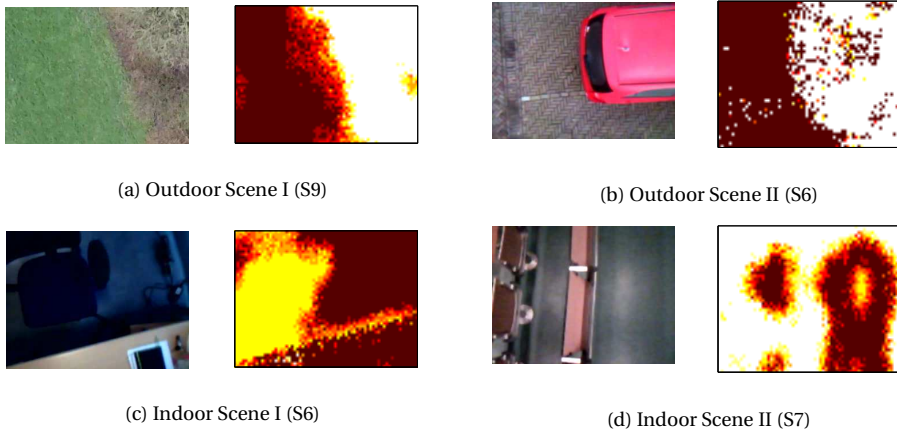
Figure 5.12: Obstacle localization using roughness \hat{e} from SSL method. The light yellow color in roughness map represents the presence of obstacles.
