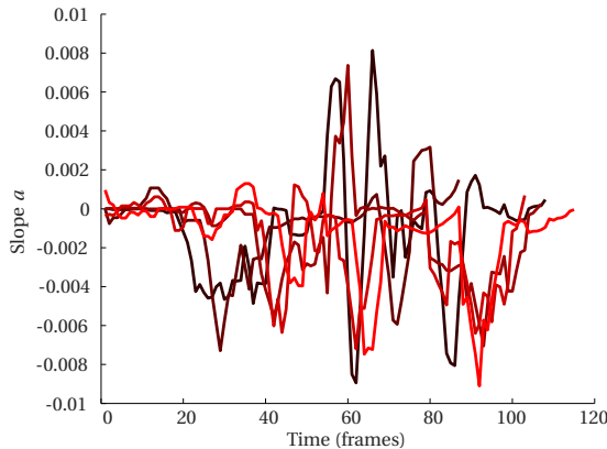
Figure 4.7: Results of slope estimation on video sequences with the camera moving in Z -direction. The plots show the estimated slope a (y-axis) over time (x-axis). The brightness of the lines are determined by the angle with the wall, with the darkest color corresponding to 0 degrees and the brightest color corresponding to 60 degrees.
