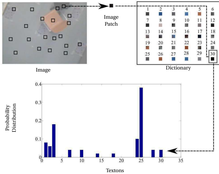
Figure 5.3: Texton Method: A number of image patches is randomly selected from an image. The patches are then compared to textons in a dictionary to form a texton probability distribution of the image.
