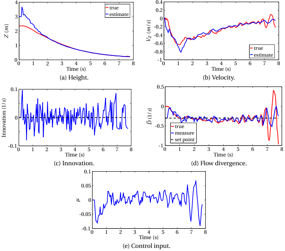
Figure 2.7: Fixed-gain landing with constant flow divergence ( D^* = -0.3 \text{ s}^{-1} ) with EKF-based height and velocity estimation.
