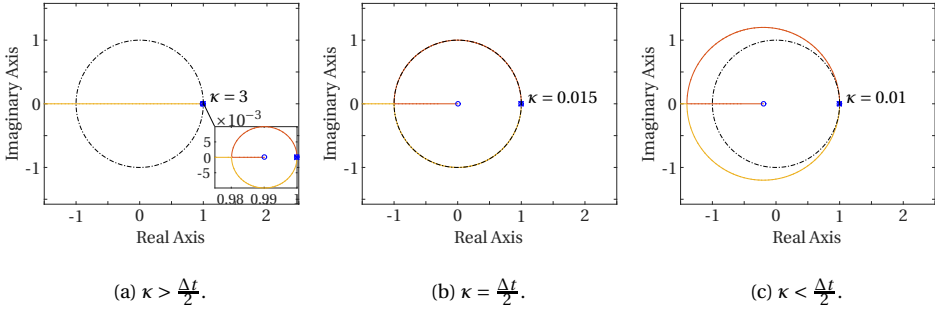
Figure 3.18: Root locus of the closed-loop discrete system for three different integral time constants.
