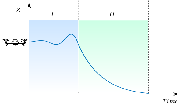
Figure 3.15: Two-phase adaptive control strategy for constant flow divergence landing. In phase I, the MAV increases the gain until it starts to oscillate. This allows the MAV to select a suitable gain for phase II, in which it lands while reducing the gain exponentially.
