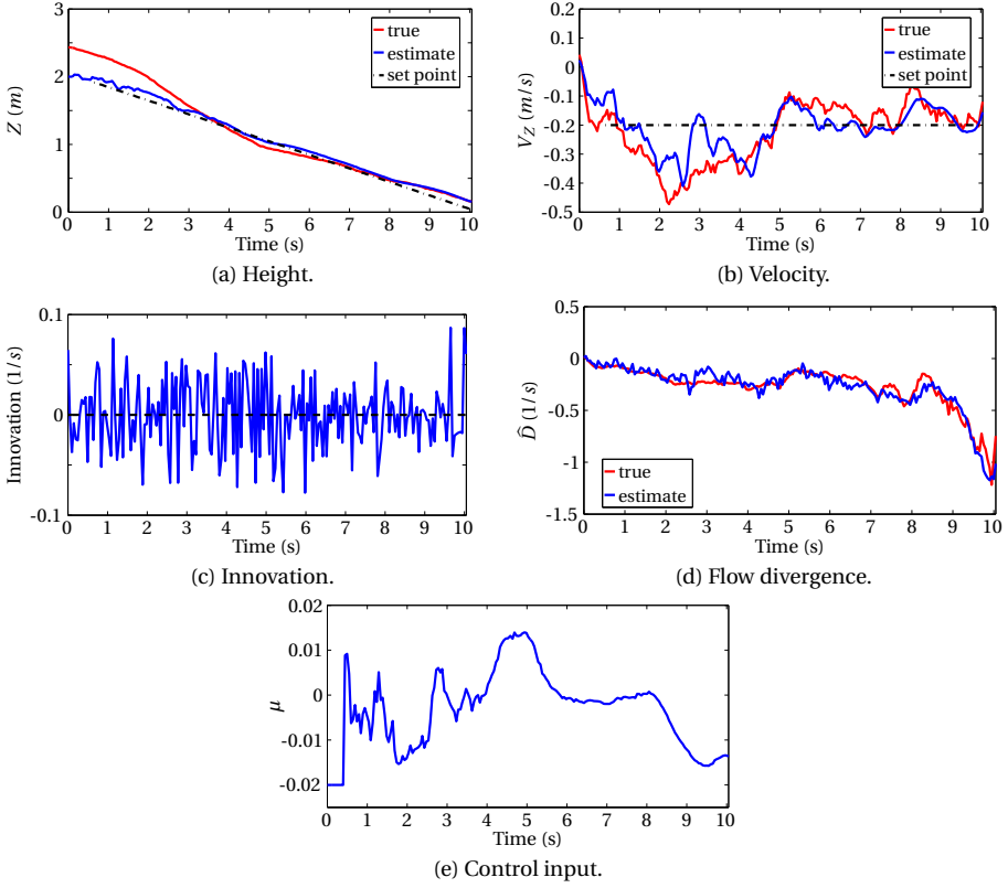
Figure 2.10: Landing with a linear controller using estimates from EKF (Indoor Flight).
