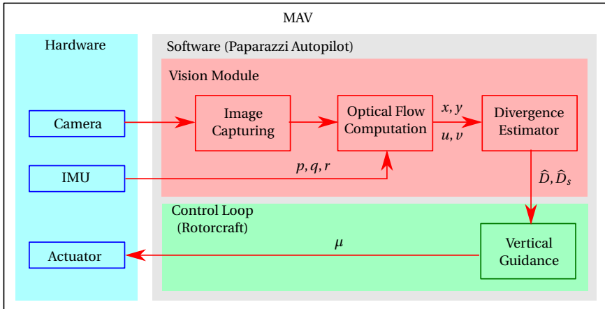
Figure 3.6: Control architecture of Paparazzi Autopilot and the integration of the computer vision module.
