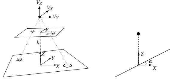
Figure 4.1: Left: the main coordinate axes involved in the optical flow calculations. Right: illustration of a ground surface with a nonzero slope \alpha .
