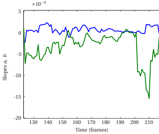
Figure 4.9: Results for estimation of slope with the Parrot AR drone's bottom camera. The plot shows a (blue) and b (green) over time ( x -axis).
