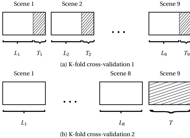
Figure 5.16: Two K-fold cross-validations for evaluation of learning and exploration capabilities of the classifier.
