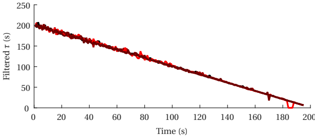
Figure 4.4: Results of time-to-contact estimation on five image zooms. The ground-truth time-to-contact goes from 200 to 5.
