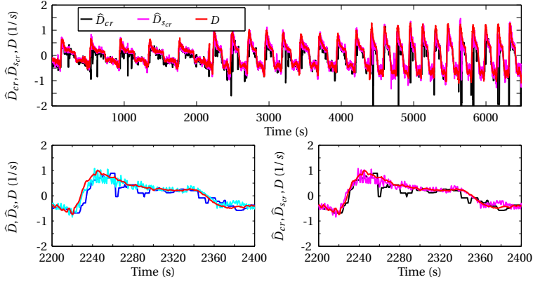
Figure 3.8: The estimated and delay-corrected flow divergences, together with their ground truth.
