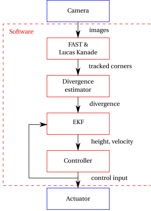
Figure 2.4: An overview of the methodology.
