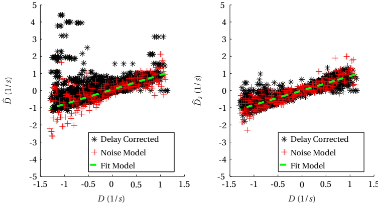
Figure 3.12: The flow divergence estimates \hat{D} (left) and \hat{D}_s (right) and the data generated using the noise models.
