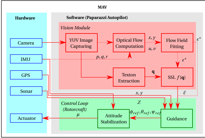
Figure 5.21: Integration of computer vision module in Paparazzi Autopilot. The left blue box shows the hardware of the MAV while the right gray box indicates the software architecture used in the MAV. The process flow guided by the dashed line can be neglected after the learning is complete.
