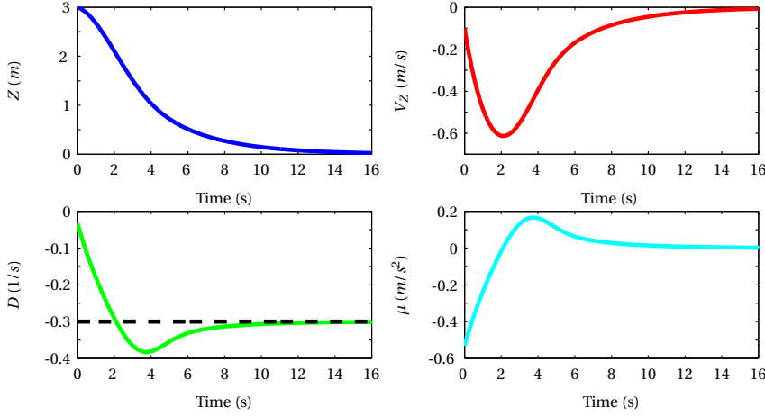
Figure 2.3: Height Z , velocity V_Z , and flow divergence D of an MAV during landing using constant flow divergence strategy ( D^* = -0.3 \text{ s}^{-1} ) with control input \mu .
