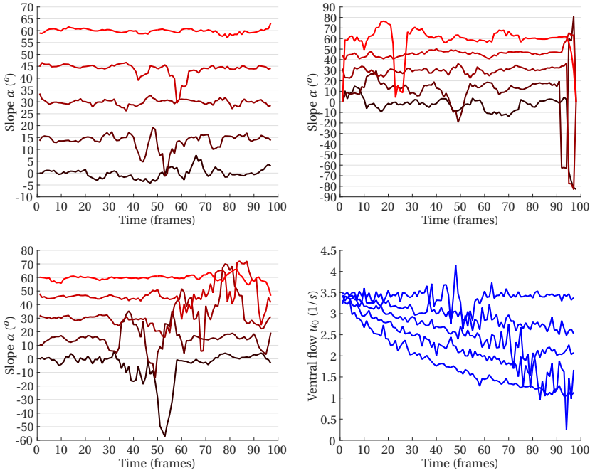
Figure 4.5: Slope estimation results on artificial movement sequences. The ground-truth values for the slopes \alpha are \{0, 15, 30, 45, 60\}^\circ . Top left: slopes estimated during movement in the Y -direction. Top right: slopes estimated during movement in the Z -direction. Bottom left: slopes estimated during movement in the X -direction. Bottom right: ventral flow \vartheta_x during movement in the X -direction.
