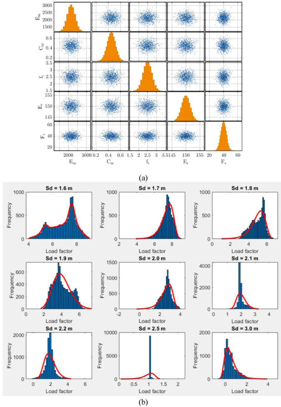
Figure 17. Parameters of the surrogate model: (a) input: MC sample of the selected random variables, and (b) output: Histogram and fitted probabilistic distribution for each scour depth ( S_d ).
