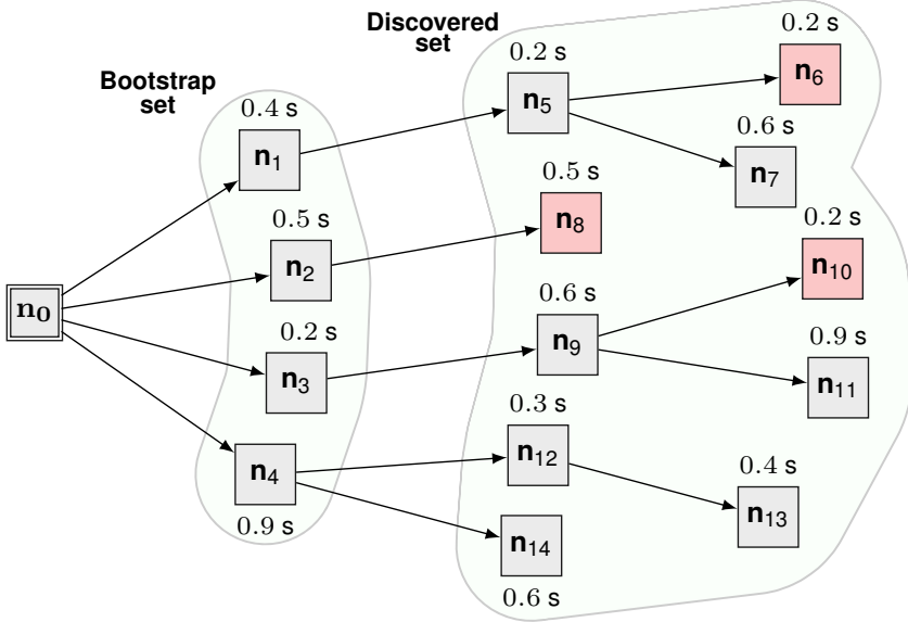
Figure 3.5: Example of a peer discovery tree for a node n_0 with a maximum depth of 3 and \Delta = 0.1 s. Nodes with dark (red) shading violate the latency diversity (i.e., their difference in latency is strictly smaller than \Delta ).
