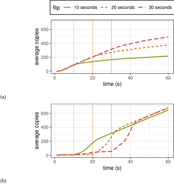
Figure 4.5: The average number of copies stored per node when at 10, 20, and 30 seconds all reputations flip from 0 to 1 (a) and 1 to 0 (b). Every node generates two records per second.
