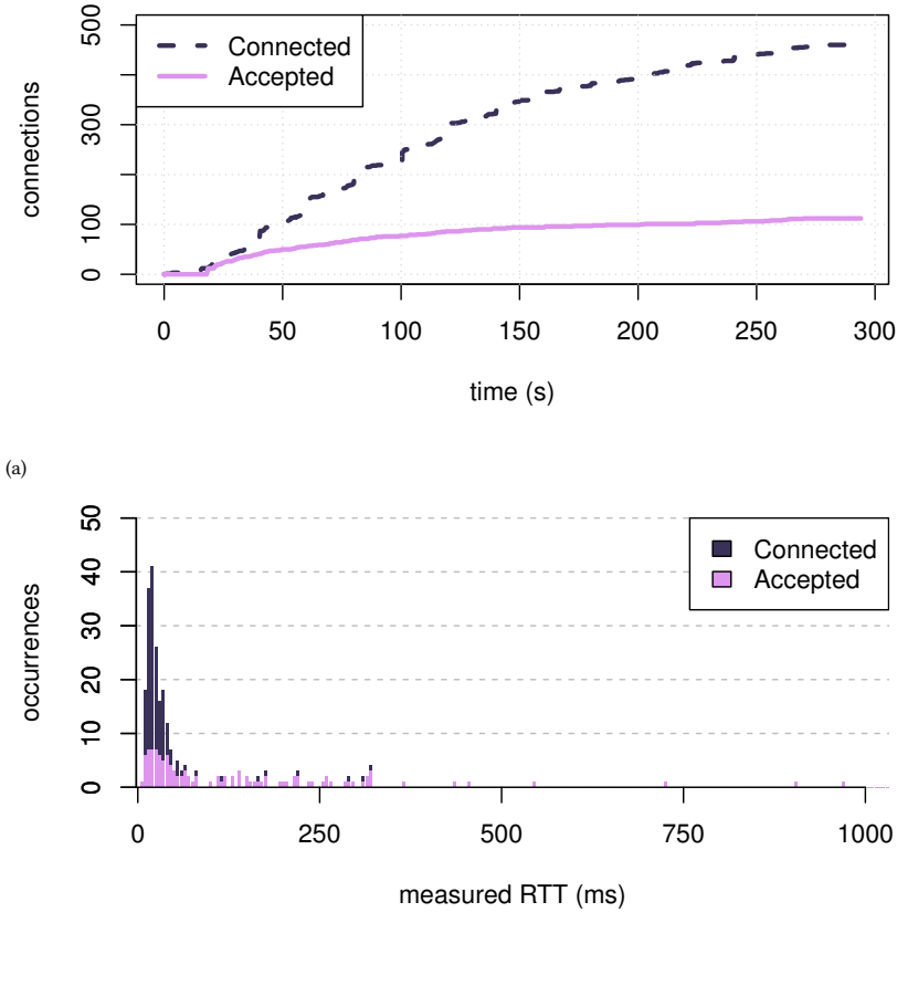
Figure 3.1: The number of connected and accepted nodes without Sybils (a) and a histogram of their latencies at the time of 300s (b).
