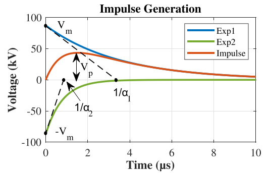
FIGURE 13. Impulse formation.
