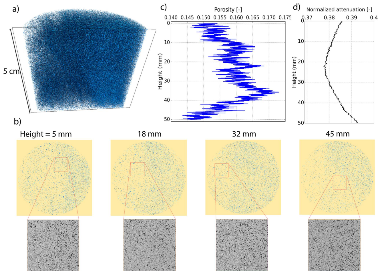
Figure 12. (a) Rendering of the X-ray tomogram of sample BS2 acquired at the European Synchrotron Radiation Facility, with a voxel size of 5.85\ \mu\text{m} . Pores are shown in blue. (b) Two-dimensional slices of porosity distribution perpendicular to the core axis at different heights including X-ray tomograph zooms of small squares, where empty pores appear in black. (c) Profile of porosity distribution along the axis of the core sample calculated by segmentation of the pores (sum of segmented pores divided by slice area), as shown in panel (a). (d) Normalized X-ray attenuation profile calculated by averaging gray values along the axis of the core sample.
