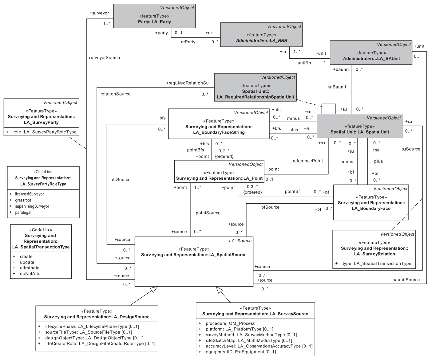
Fig. 8. Classes and subclasses of the LA_Source and integrated source.
