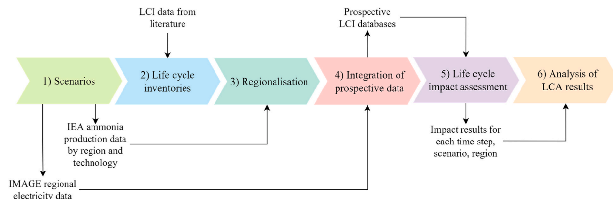
Fig. 1. Method overview.
