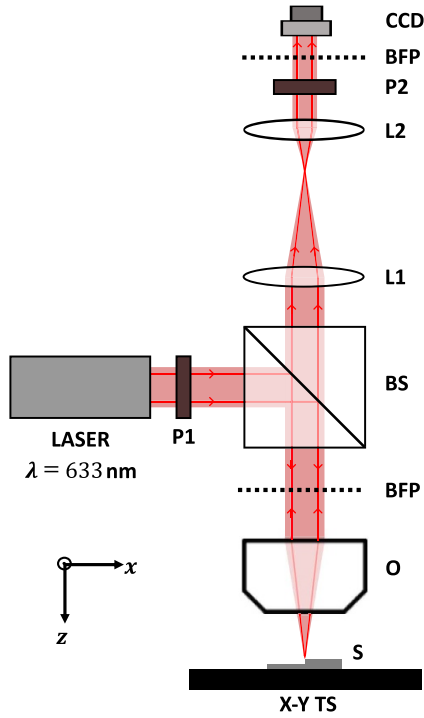
Figure 2. Schematic of the experimental setup of coherent Fourier scatterometry (CFS).
