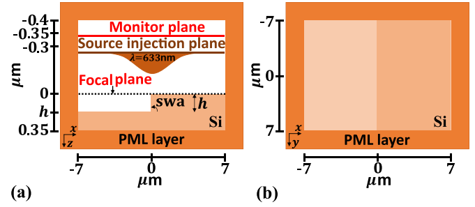
Figure 3. The 3D-FDTD simulation scheme of a cliff-like nanostructure characterized by geometrical parameters: swa and h , being illuminated by a TE or TM polarized focused spot of wavelength 633 \text{ nm} . The corresponding y = 0 plane in (a). The corresponding z = 0 plane in (b).
