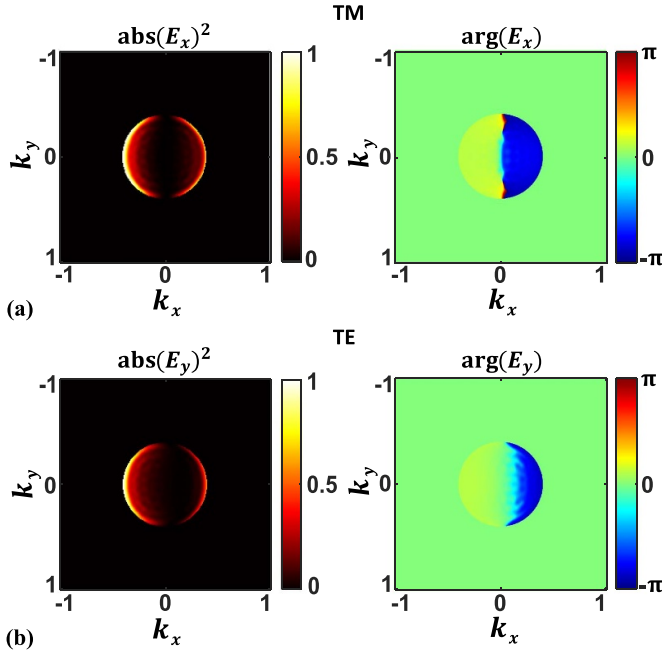
Figure 4. (a) Simulated normalized far-field intensity (on the left) and phase (on the right) for a cliff-like nanostructure with geometrical parameters: \text{swa} = 90^\circ and h = 150 nm, being illuminated by a TM polarized focused spot having \lambda = 633 nm. (b) Corresponding far-field intensity (on the left) and phase (on the right) for the same nanostructure illuminated by a TE polarized focused spot having \lambda = 633 nm.
