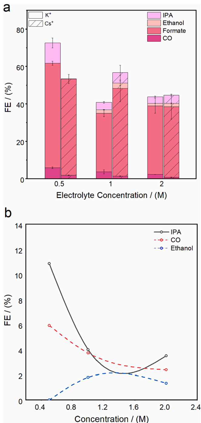
Fig. 5. a) fe of co, ethanol, hcooh, and isopropanol versus electrolyte concentration (0.5, 1, and 2 M) at P = 25 bar and -9.1 \text{ mA/cm}^2 , b) Relationship between \text{FE}_{\text{IPA}} , \text{FE}_{\text{CO}} , and \text{FE}_{\text{EtOH}} versus \text{KHCO}_3 concentration at j = -9.1 \text{ mA/cm}^2 and P = 25 bar.
