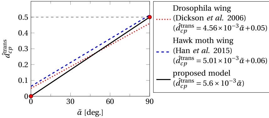
Figure 2.6: Measured chordwise centre of pressure (CP) for dynamically scaled insect wings and the analytical formula of CP used in our model. The values of CP are normalized by local chords and denoted as \hat{d}_{cp}^{trans} .
