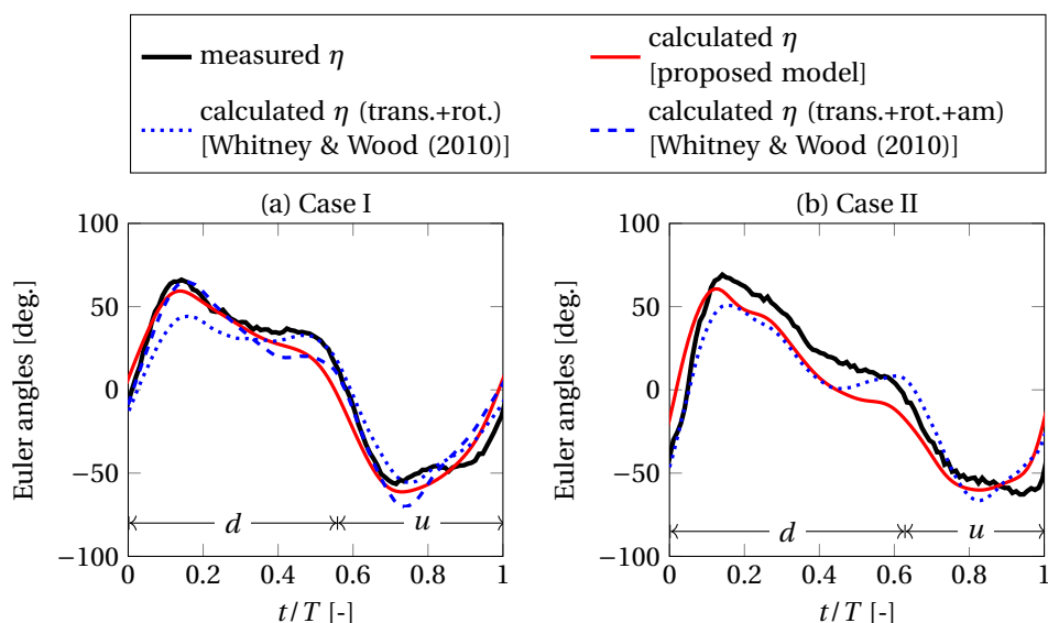
Figure 2.20: Comparison of the passive pitching motion predicted by the proposed quasi-steady model and the model of Whitney & Wood (2010) for both cases.
