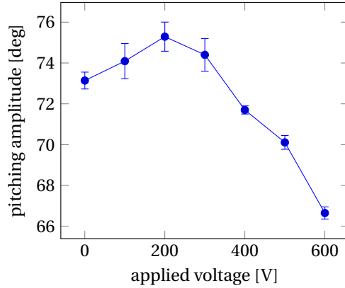
Figure 5.13: Average pitching amplitude as a function of the applied voltage V . The error bars indicate the measurement uncertainty as determined by the non-smoothness of the measured pitching motion \eta(t) .
