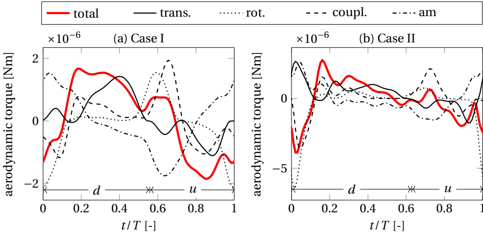
Figure 2.19: Total aerodynamic torque and its components induced by the wing translation, rotation, the coupling term as well as the added-mass effect for both cases.
