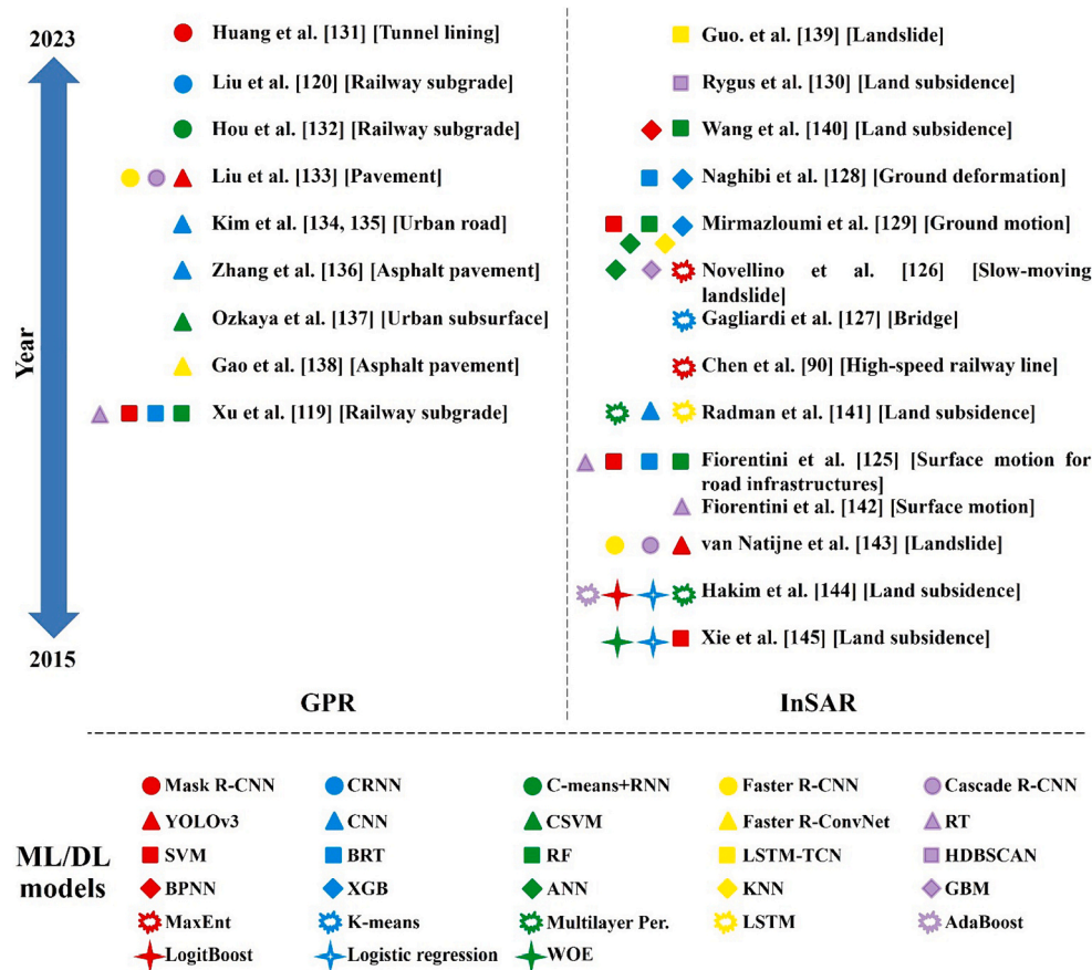
Fig. 8. Illustrative layout of ML models incorporated in InSAR/GPR for civil engineering infrastructures [90,119,120,125–145].
