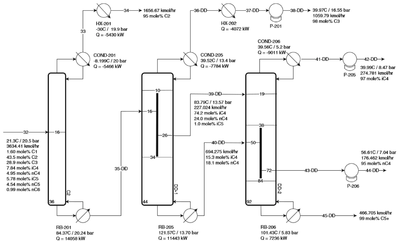
Fig. 4. NGL fractionation PFD of DDWCs (Configuration 2.2).
