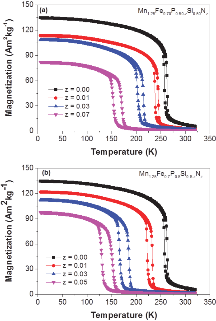
Figure 6.8: Magnetization curves measured on heating and cooling in a magnetic field of 1 T for the \text{Mn}_{1.25}\text{Fe}_{0.70}\text{P}_{0.5-2}\text{Si}_{0.5}\text{N}_2 (a) and \text{Mn}_{1.25}\text{Fe}_{0.70}\text{P}_{0.5}\text{Si}_{0.5-2}\text{N}_2 (b) compounds.
