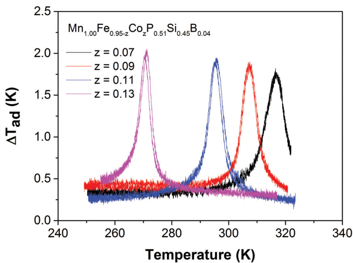
Figure 7.10: Temperature dependence of the adiabatic temperature change obtained by direct measurements for the \text{Mn}_{1.00}\text{Fe}_{0.95-z}\text{Co}_z\text{P}_{0.51}\text{Si}_{0.45}\text{B}_{0.04} compounds in a magnetic field change of \Delta B = 1.1 T.
