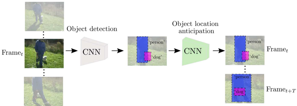
Fig. 1.3: Chapter 2: Efficient video object detection. The proposed video object detection method starts from individual video frames at timestep t and detects the object locations via a convolutional neural network (CNN). Subsequently, the novelty of the method comes from anticipating the future object locations (highlighted in green, here) over the next T frames. Thus, the frames between timestep t and t+T do not need to be processed in the network, leading to efficiency.
