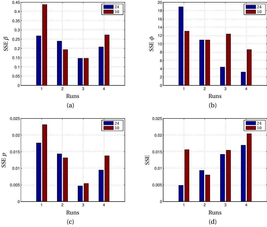
Figure 5.12: Comparing the minimum model size with the maximum size (10 and 24 independent variables) for the SSE over the trajectory up to the final roll. The failure is a partial loss of aileron.
