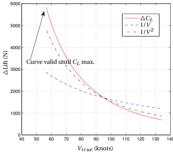
Figure A.2: Additional lift caused by propeller slipstream for the PA-34 using maximum power. Graph only valid until maximum C_L is reached. The 1/V and 1/V^2 curves are 'anchored' to the \Delta L at 97.2 knots.
