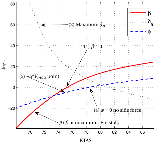
Figure 3.10: PA-34 Right Engine Inoperative, Left Engine Maximum Power and Rudder Full Left.
