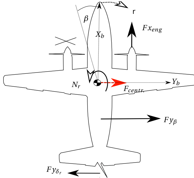
Figure 3.2: Forces in a flat turn into the operative right engine with \phi = 0 and left engine inoperative.
