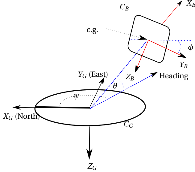
Figure 3.1: Geographic Coordinate system C_G and Body Coordinate system C_B . Both coordinate systems are displaced for clarity, which can be done because only the relative orientation is important and not their relative position.
