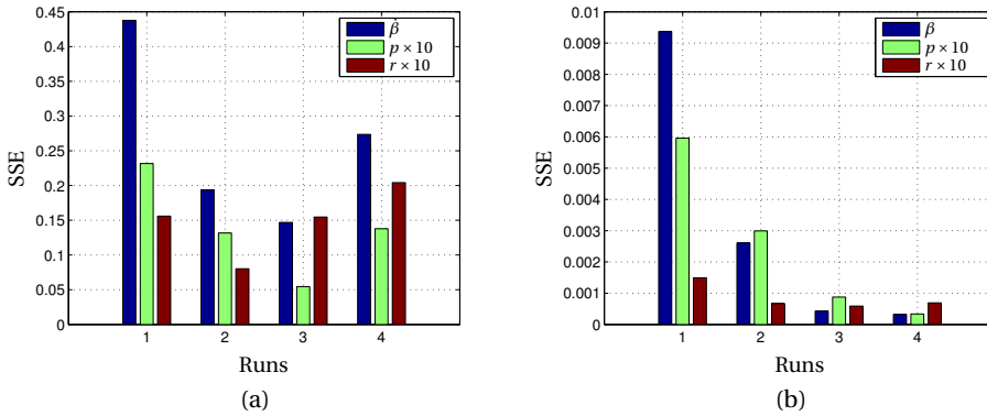
Figure 5.11: Effect of data size (multiple runs) on SSE for 24 parameter model. The multiple runs do not include data from the final roll. Runs are for a partial aileron failure in smooth and turbulent conditions with different types of inputs. (a) is SSE for trajectory up to the final roll and (b) is the SSE of the predicted final roll.
