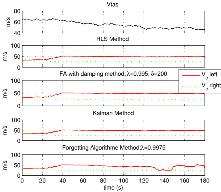
Figure 6.9: Engine failure, comparing different PID methods for run 143 in turbulence conditions, model with 22 variables, initial parameter values based on 120 knots and modified normalization.
