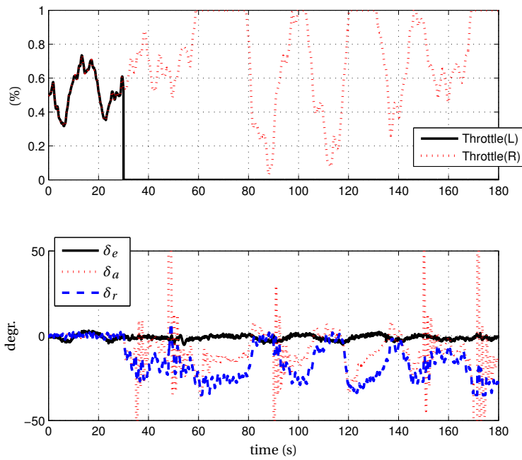
Figure 6.5: Inputs in initial model parameter values profile. The profile shows a left engine failure (Run 111) in turbulent conditions at an average true airspeed of 85 knots.
