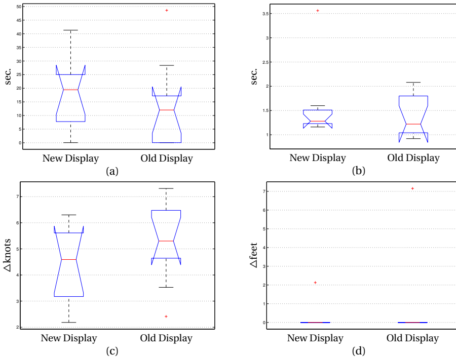
Figure 8.15: Engine Failure after take off (EFATO), results of different display types in the first run. (a) the needed recovery time to velocity >88 KIAS, (b) the time required to achieve full rudder, (c) the maximum airspeed loss in knots and (d) the altitude loss if present; most pilots did not experience any altitude loss consequently, the box plot is compressed to a line.
