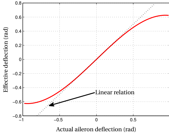
Figure 5.15: Aileron effectiveness PA-34 based on Eq. 5.44.
