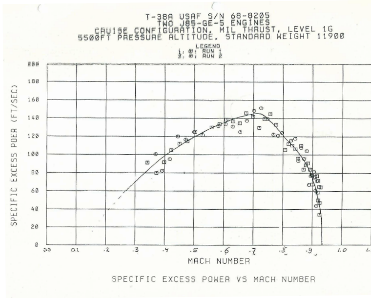
Figure 2.1: Specific Excess Power T-38 at 5000'; Test performed by author at USAF TPS 1984
