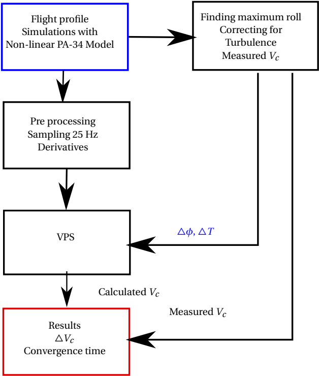
Figure 6.6: Graphic representation of the V_c test.
