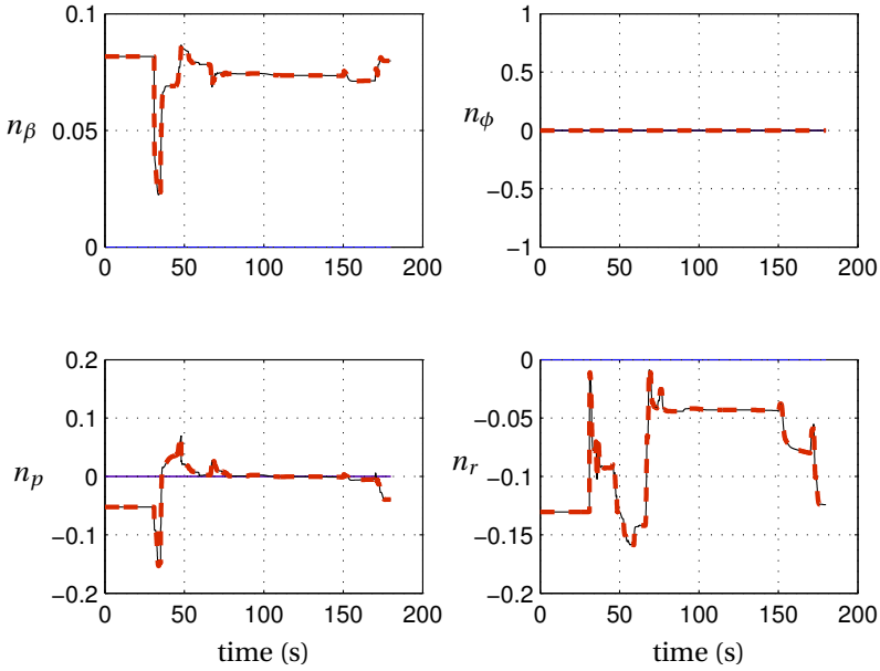
Figure 6.12: PID result model parameters during a Rudder Hard-over; MKM method; resetting by multiplying the covariance matrix by 10,000.
