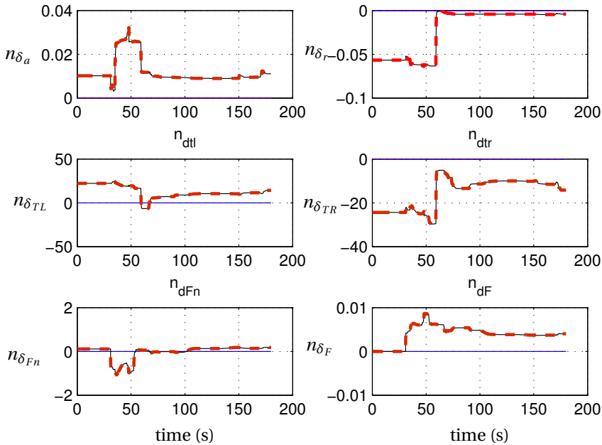
Figure 6.11: PID result state parameters during a Rudder Hard-over; MKM method; resetting by multiplying the covariance matrix by 10,000.
