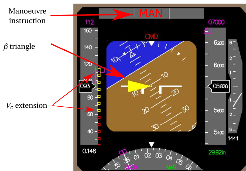
Figure 7.2: The PFD used in the experiments, augmented with (1) V_c indicator and (2) a centred side slip display that can either display \dot{y} in white or \beta in yellow. The Manoeuvre instruction is displayed for 15 seconds after the detection of a failure.
