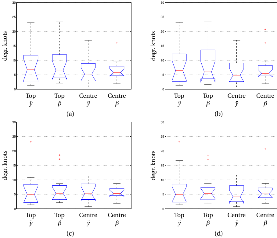
Figure 8.5: The total scores over the complete trajectory are compared for different numbers of pilots and for the effect of the omission of the first run. (a) All runs 16 pilots, (b) All runs 19 pilots, (c) Runs 2, 3 and 4 using 16 pilots and (d) Total score 19 pilots over runs 2, 3 and 4.
