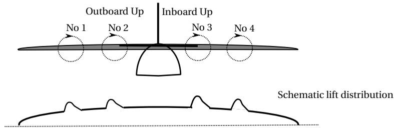
Figure A.4: Rear view of the C-130 with propeller numbers, propeller turn direction and schematic lift distribution over the wing due to propeller slipstream effect.
