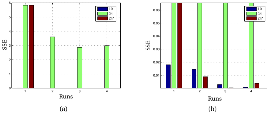
Figure 5.16: Prediction accuracy in SSE ( \phi ). Comparing (1) the 10 parameter model using the linearised aileron, with (2) the 24 parameter model and the non linear aileron and (3) the same set as (2) but with incorporation of the final roll in the parameter estimation. Figure (a) shows the normal view and Figure (b) shows the expanded view.
