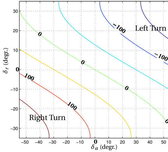
Figure 3.3: Available initial roll rate acceleration in \text{deg./s}^2 , for PA-34 with gear and flaps up. No thrust asymmetry, 85 KTAS and altitude 300m. (Positive control deflection is left rudder and left aileron.)
