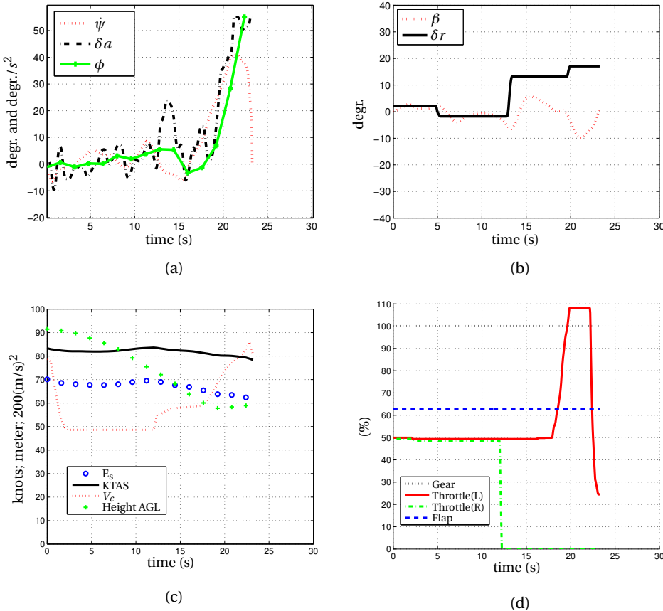
Figure 7.7: Effect of a rapid throttle input with delayed rudder response; (a) Heading rate, roll angle and roll inputs, (b) Side slip and rudder inputs, (c) Energy management with KTAS, height (m) and total specific energy ( E_s ) in units of 200(m/s)^2 and (d) Throttles, flap and gear at % of their maximum values
