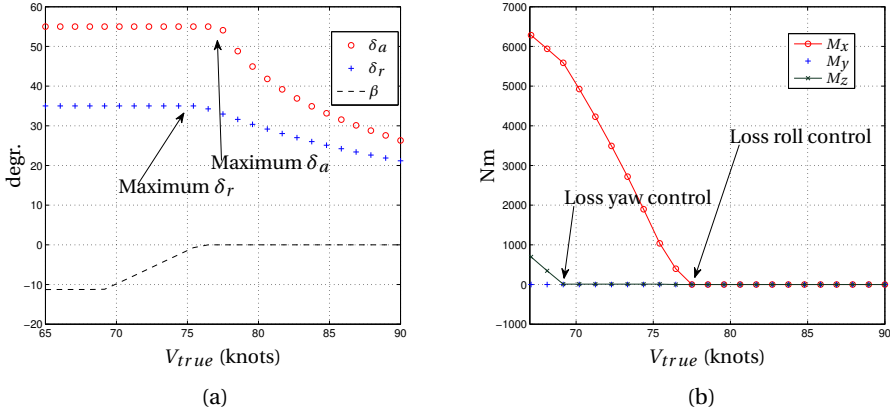
Figure 3.5: Trim conditions PA-34. \beta = 0 until maximum \delta_r is reached, \phi is adjusted to maintain heading as long as enough aileron is available. Flap=25°; Gear up; Trimmed for maximum climb with right engine failed; (a) Control deflections (b) Aerodynamic moments in body coordinate system.
