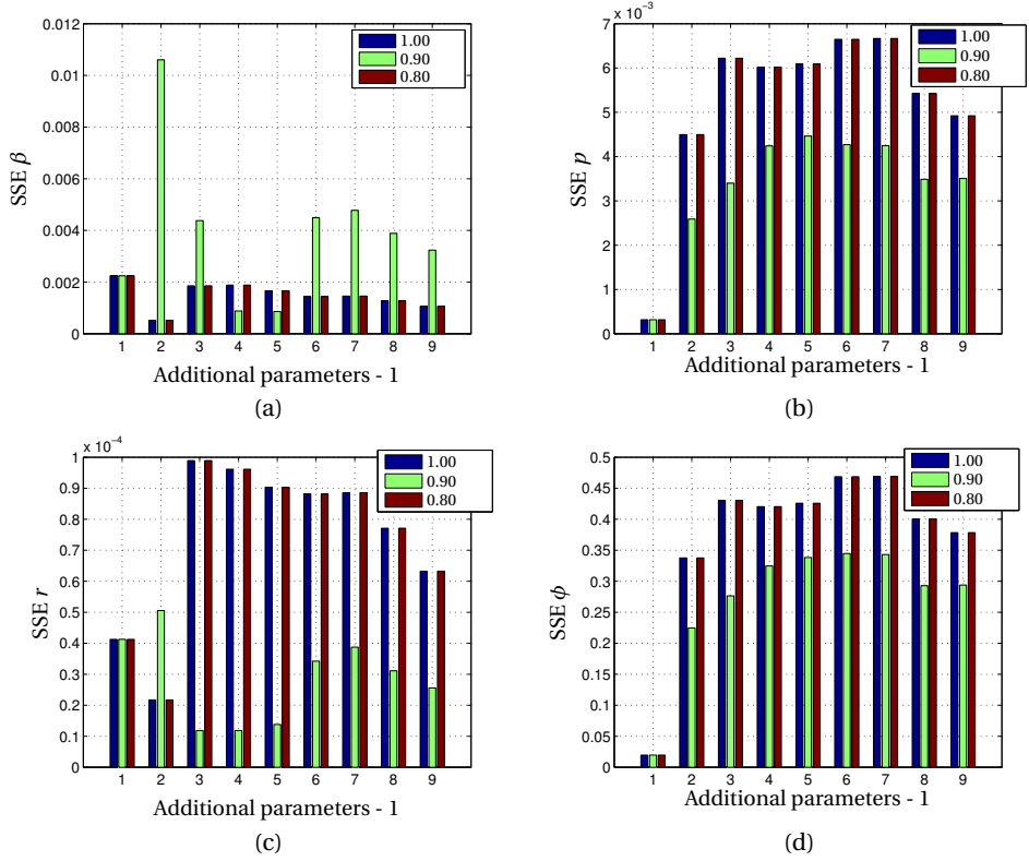
Figure 5.10: The effect of adding a collinearity check on the AICC method. The chosen run (177) is a lateral asymmetry in smooth flying conditions; Three limits were investigated: 1.0, which equates to no limit, 0.9 maximum collinearity and 0.8 maximum collinearity. The figures present the SSE of the final roll as function of additional parameters. Figure (a) is SSE \beta , (b) is SSE p and (c) is SSE r and (d) is SSE \phi over the complete run.
