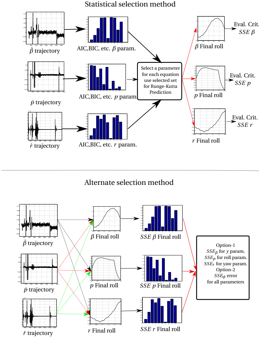
Figure 5.4: Comparison between normal and alternate selection process.
