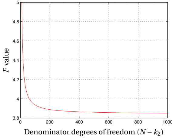
Figure 5.5: Relation between F value and (N - k_2) for a probability of 95% and k_2 - k_1 = 1 .
