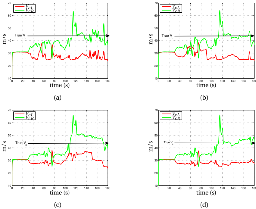
Figure 6.3: Comparison of different \lambda values for the FA method; The run is done with a PA-34 in turbulent flying conditions with an asymmetry failure at 30 seconds in the flight. The run details are described in Section 6.3. The true V_c value after the failure is 44 m/s. In red the V_c for a left roll ( V_{cL} ) and in green V_{cR} for a right roll. (a) \lambda = 0.9925 ; (b) \lambda = 0.995 ; (c) \lambda = 0.9975 (d) \lambda = 0.9995 .
