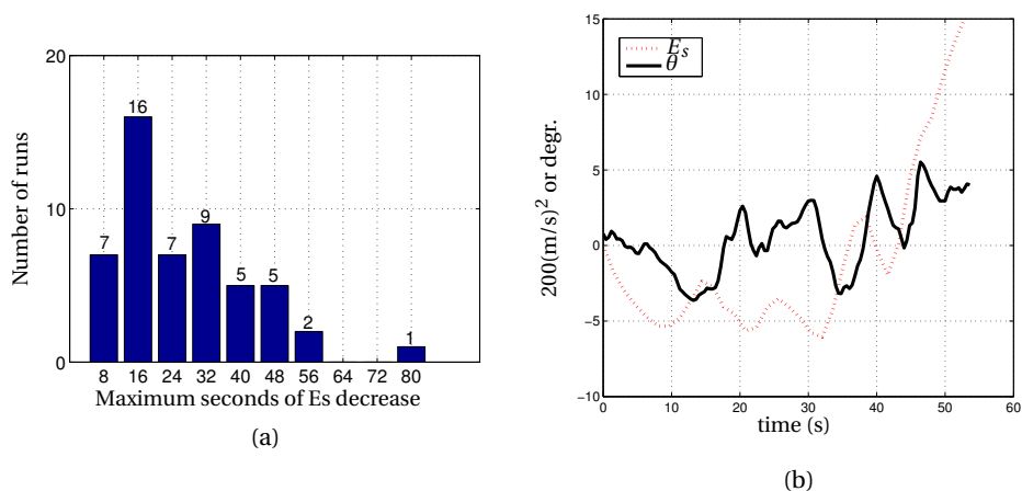
Figure 7.8: (a)Histogram of 52 go-around runs; Total time of energy decrease after initiating go-around and (b) Example of total energy and \theta control in run 194; The specific total energy is off-set in y-axis for clarity: E_s at the start of the run is set to 0.
