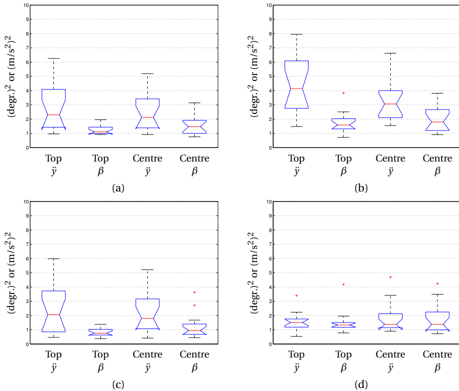
Figure 8.6: Slip variance for the different slip displays in the OEI climb; Variance in slip is for \beta in degrees^2 and for \ddot{y} in (0.1m/s^2)^2 depending on the kind of display. (a) Represents the score over the complete trajectory, (b) represents the score for the initial part of the climb, (c) is the score over the steady part of the climb and (d) is the level off part.
