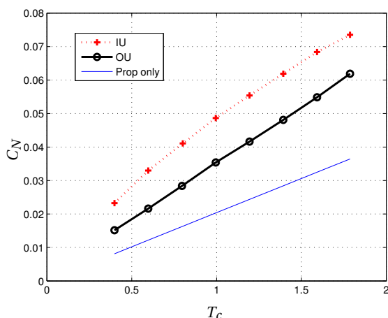
Figure A.3: Mannée [5]: Effect T_c on C_N for Inboard Up (IU) and Outboard Up (OU) turning propellers compared to the effect without vertical tail for a high wing configuration
