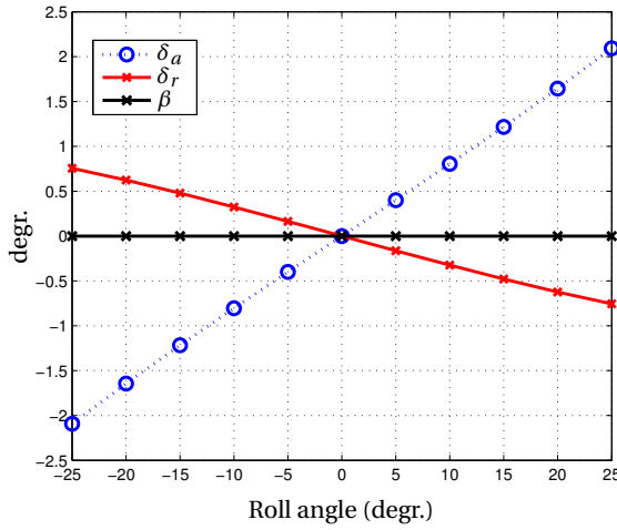
Figure 3.8: Required aileron en rudder deflection to maintain a level turn for the PA-34 at zero side slip angle, flying at 80 KTAS.
