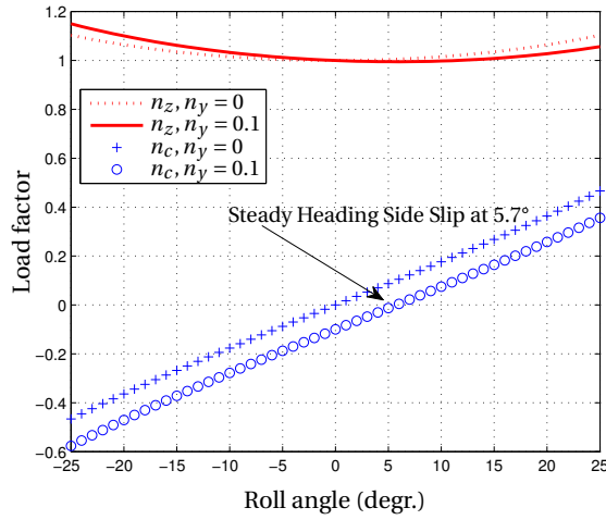
Figure 3.7: Effect of roll angle on lift and centripetal force with a constant side force due to \beta that is 0.1mg , based on Eq. 3.9.
