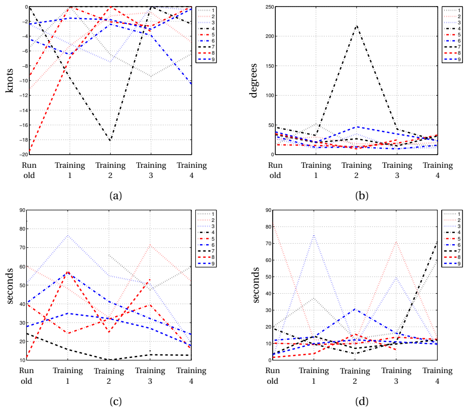
Figure 8.14: Subjects learning curves in OEI go-around training. (a) maximum \Delta V_c , (b) Maximum bank angle excursion in degrees (c) the recovery time and (d) time minimum energy is reached after the engine failure.
