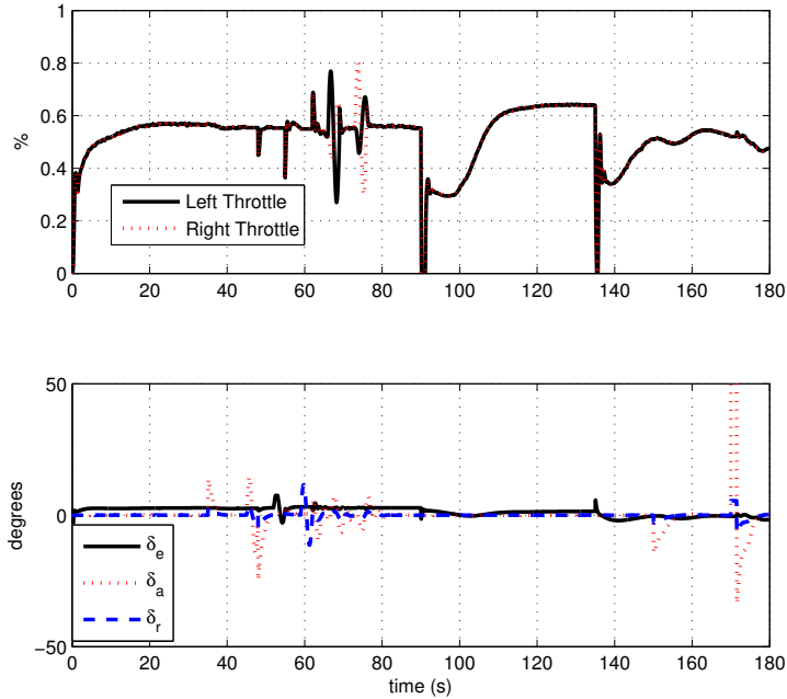
Figure 6.8: Control inputs during failure profile. Shown profile is a partial (50%) aileron failure
