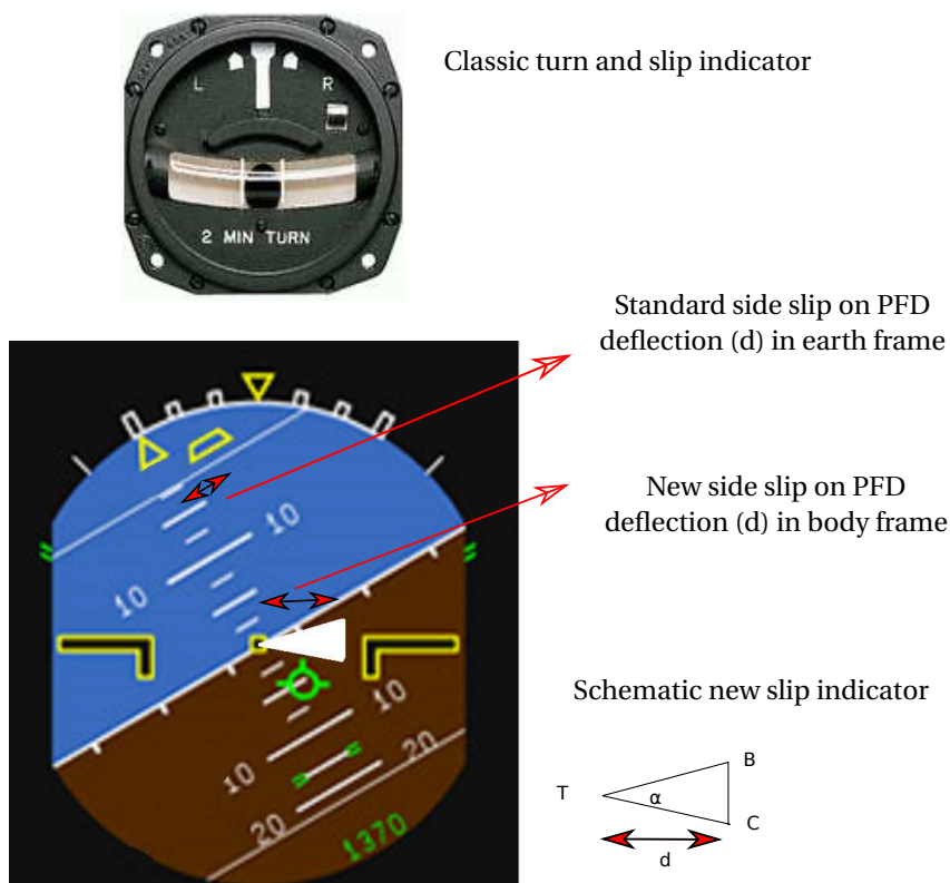
Figure 7.1: Different Side Slip indicators
