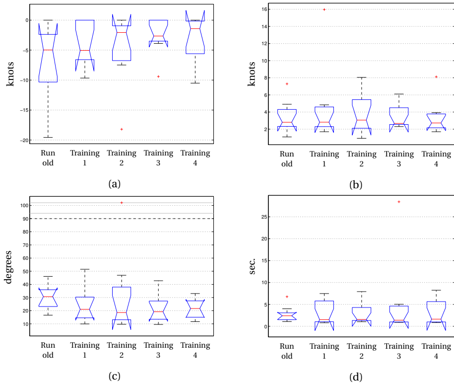
Figure 8.12: Safety related parameters in OEI go-around during training session. (a) The V_c exceedance, (b) the maximum velocity decrease after the engine failure (c) the maximum bank angle and (d) the time required to get maximum rudder deflection.
