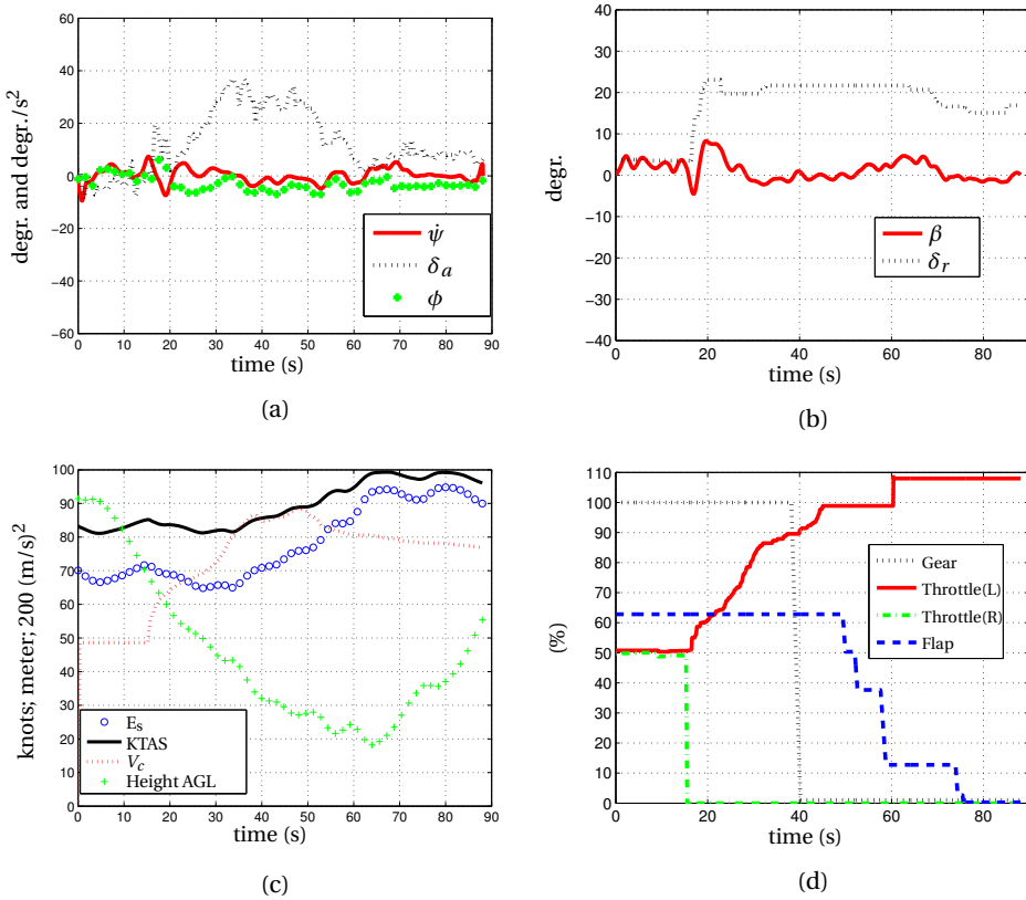
Figure 7.6: Typical well executed go-around with (a) Heading rate, roll angle and roll inputs, (b) side slip and rudder inputs, (c) Energy management with KTAS, height (m) and total specific energy ( E_s ) in units of 200(m/s)^2 and (d) Throttles, flap and gear, shown as percentage of their maximum values.
