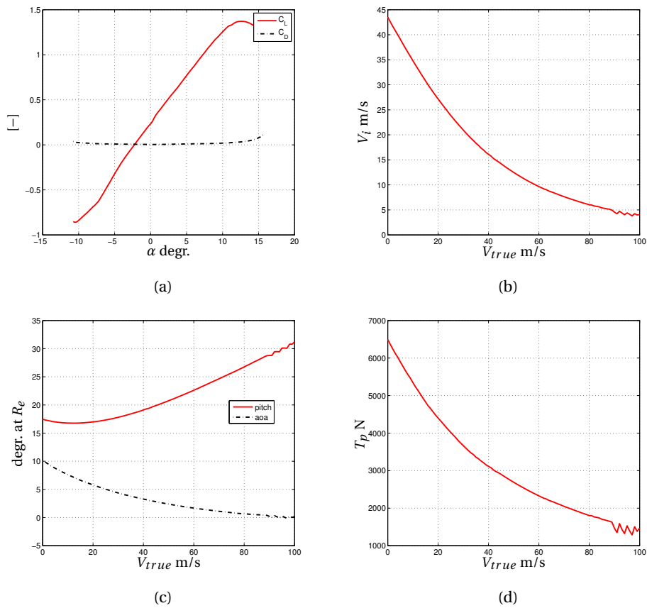
Figure B.2: Result simulation with propeller blade element program for the data of Table B.1; (a) C_D and C_L for NACA 5406; (b) Induced velocity in slipstream; (c) AoA and pitch change at R_e , (d) Thrust.
