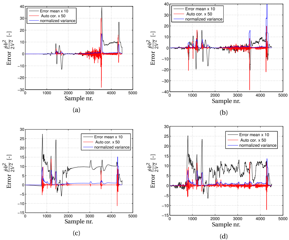
Figure C.3: Mean, Auto correlation and variance error in roll channel for different runs: (a) 50% aileron failure in smooth flying conditions, (b) non failure profile in turbulent flying conditions, (c) engine failure in smooth flying conditions and (d) engine failure in turbulent flying conditions.
