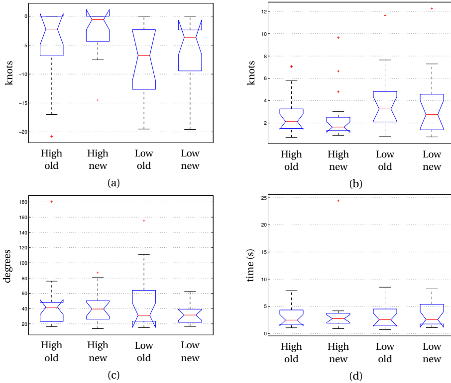
Figure 8.9: Safety related parameters in OEI go-around. (a) The V_c exceedance, (b) the maximum velocity decrease after the engine failure (c) the maximum bank angle and (d) the time required to get maximum rudder deflection.
