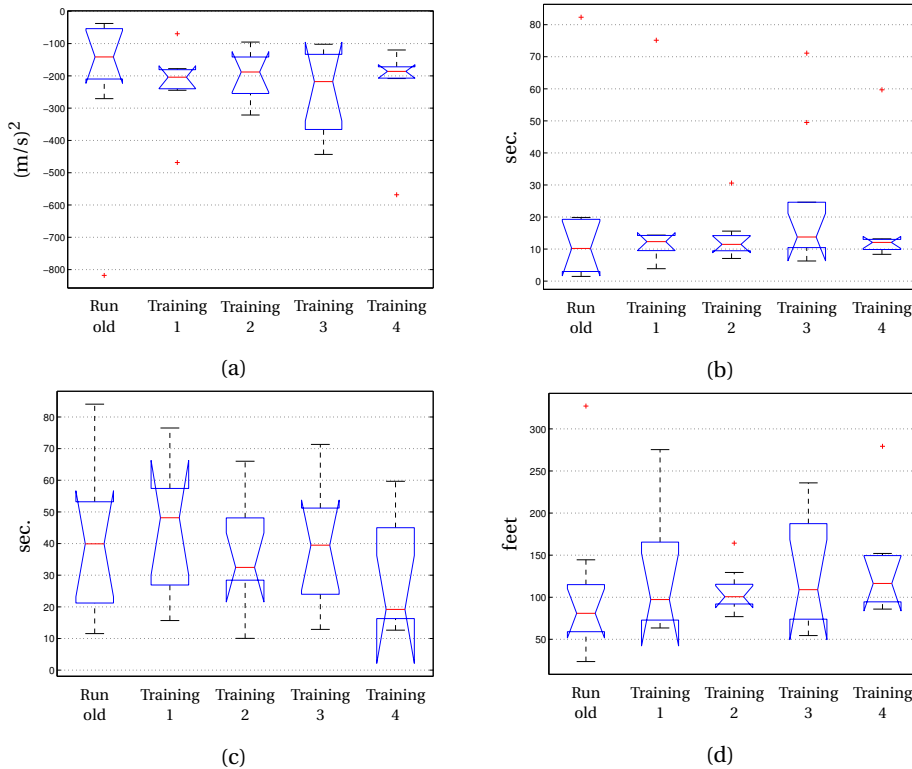
Figure 8.13: Efficiency related parameters in OEI go-around training. (a) Minimum specific energy since engine failure, (b) Time minimum energy is reached after the engine failure (c) the recovery time, which is defined as the time from engine failure until the aircraft has a speed above 85 knots with gear and flaps up; (d) the maximum altitude loss after the engine failure.
