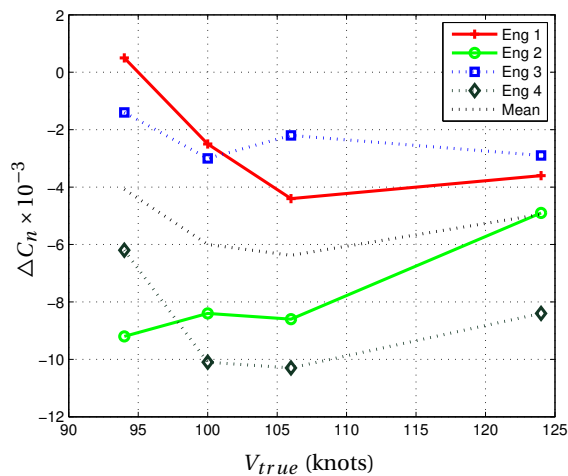
Figure A.5: The cross flow effect as function of the failed engine and V_{true} . Data based on a test flight with a RNLAf C-130H in 2002. The Hercules has right turning propellers, consequently the left engines (1 and 2) are OU and the right engines (3 and 4) are IU.
