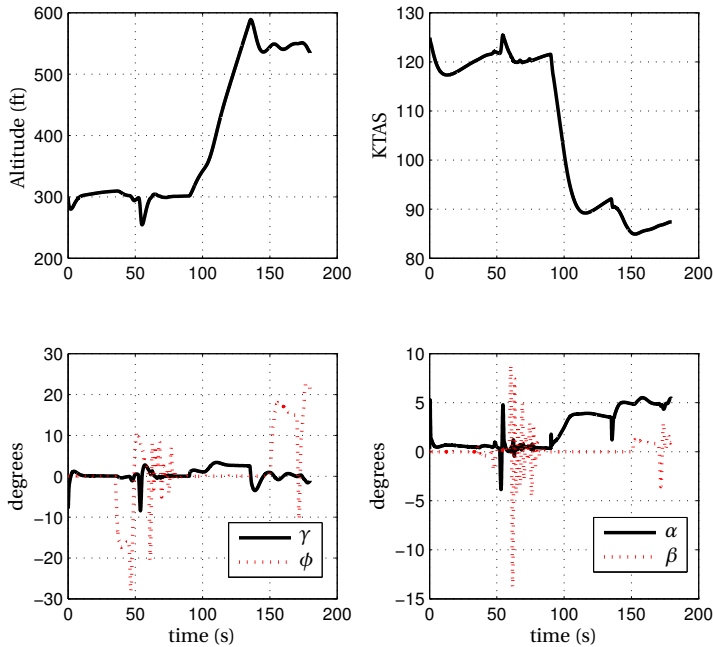
Figure 6.7: Typical Failure profile; 50% Aileron Failure in smooth flying conditions.
