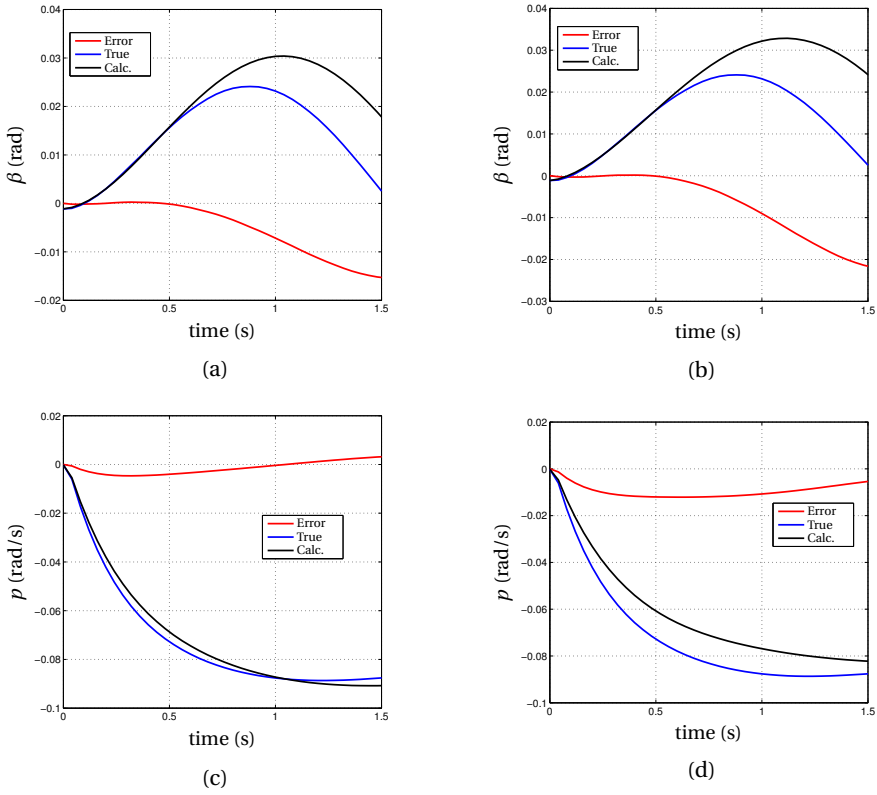
Figure 5.7: Comparison between the calculated \beta and p in the final roll manoeuvre, based on the derived model parameters, using a Runge Kutta integration and the actual \beta and p values. The chosen run is a lateral asymmetry in smooth flying conditions; (a) initial \beta errors, (b) final \beta errors after 5 additional model parameters were added, (c) initial p errors (d) final p errors after 10 additional model parameters were added. The AICC criterion was used for selecting additional model parameters.
