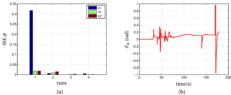
Figure 5.14: Figure (a) shows the SSE of \phi for the predicted roll using the 24 and 10 independent variables. The final roll is included in the first two data sets. For comparison the SSE of \phi without the final roll, using the 10 parameter set is included and marked as 10*. Figure (b) shows typical aileron inputs used in each run.
