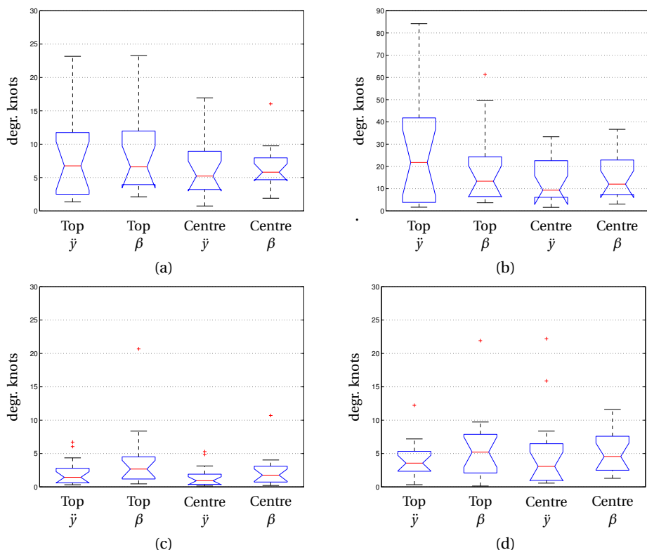
Figure 8.4: Scores for the different slip displays in the OEI climb; Scores are calculated by multiplying the absolute speed error in knots with the absolute heading error in degrees and taking the time average over the climb trajectory. (a) Represents the score over the complete trajectory, (b) represents the score for the initial part of the climb, (c) is the score over the steady part of the climb and (d) is the level off part. The large errors in the initial part necessitate a different scale for (b).
