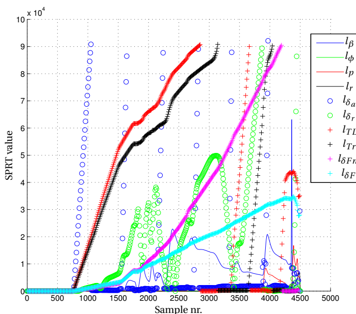
Figure C.2: Effect of individual parameter resets for SPRT SL, run is lateral asymmetry of the Citation aircraft in smooth flying conditions [6].
