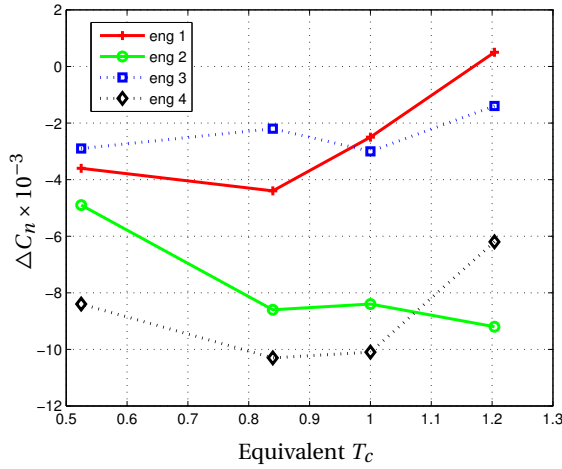
Figure A.6: The cross flow effect caused by failing one engine as function of equivalent T_c . The \Delta C_n is calculated by subtracting the engine moment from yaw moment based on \delta_r . Data are based on a test flight with a RNIAF C130H in 2002
