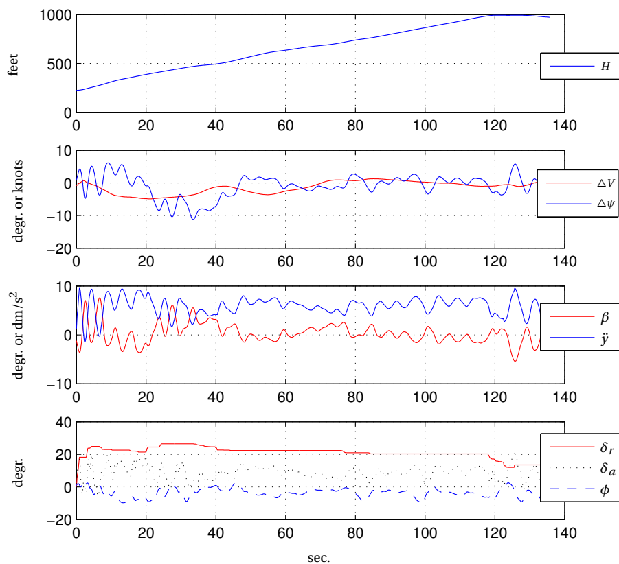
Figure 8.3: One-engine-inoperative (OEI) climb profile (run 614) where the pilot is using the triangle shape \beta display.
