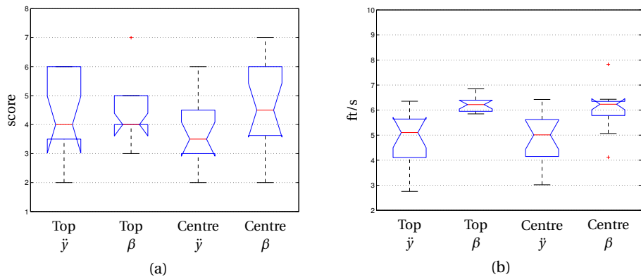
Figure 8.7: Workload and climb rate using different displays in the OEI climb. (a) represents the workload using the Bedford scale and (b) represent the average climb rate in ft/s
