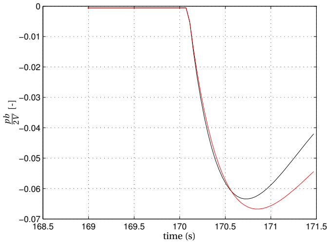
Figure 6.14: Rudder Hardover run 41; Reconstruction of final maximum deflection roll. In red the reconstruction of the roll and in black the actual roll.
