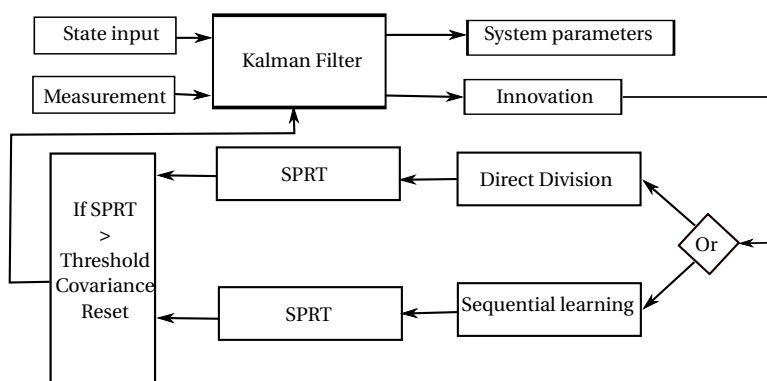
Figure C.1: Block diagram of the concept.
