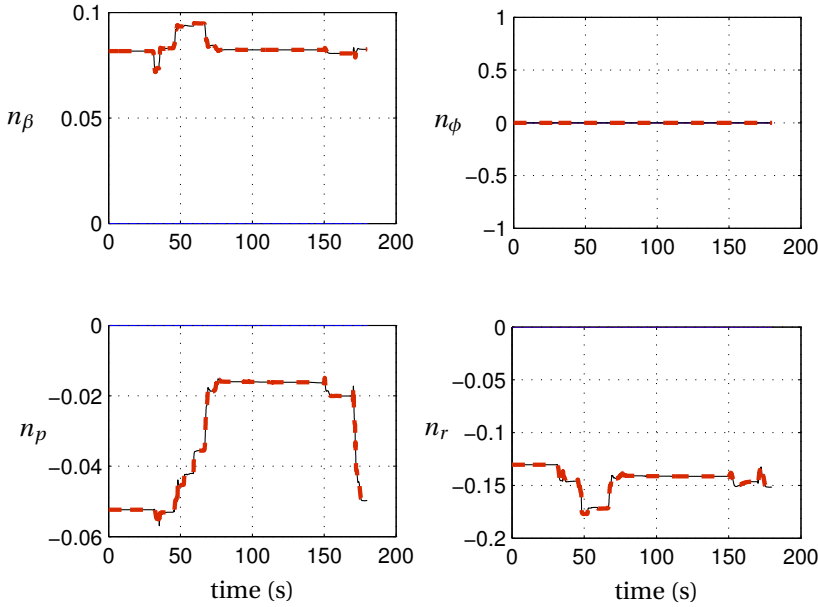
Figure 6.13: Determination of roll control parameters during a Rudder Hardover; MKM method; resetting by setting covariance matrix to fixed values.
