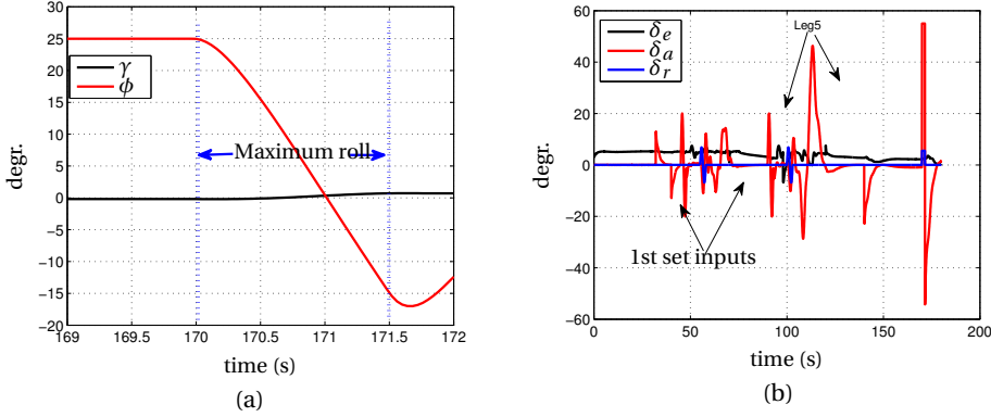
Figure 5.3: Flight profile used, (a) the maximum rate roll at 170 sec, used as evaluation criterion, (b) inputs from a run with a double set of inputs. In runs with a single set of inputs the second set, starting at 90 sec. is omitted.
