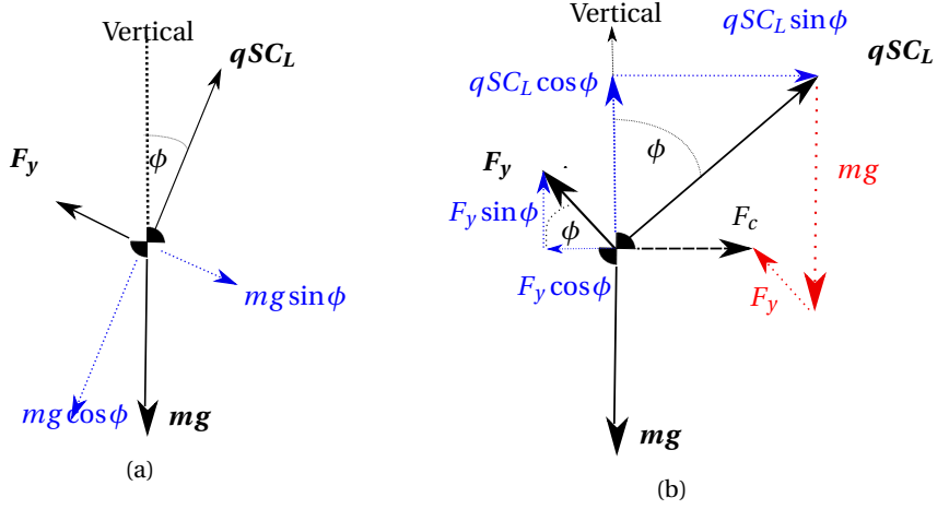
Figure 3.6: Aircraft with side force due to \beta ; Aircraft X_B axis is pointing into the paper and \theta = 0 ; (a) In a Steady Heading Side Slip and (b) In a turn where the sum of Lift, mg and F_y results in a centripetal force F_c . In red the laterally displaced vectors, in blue the vector components as a function of \phi .
