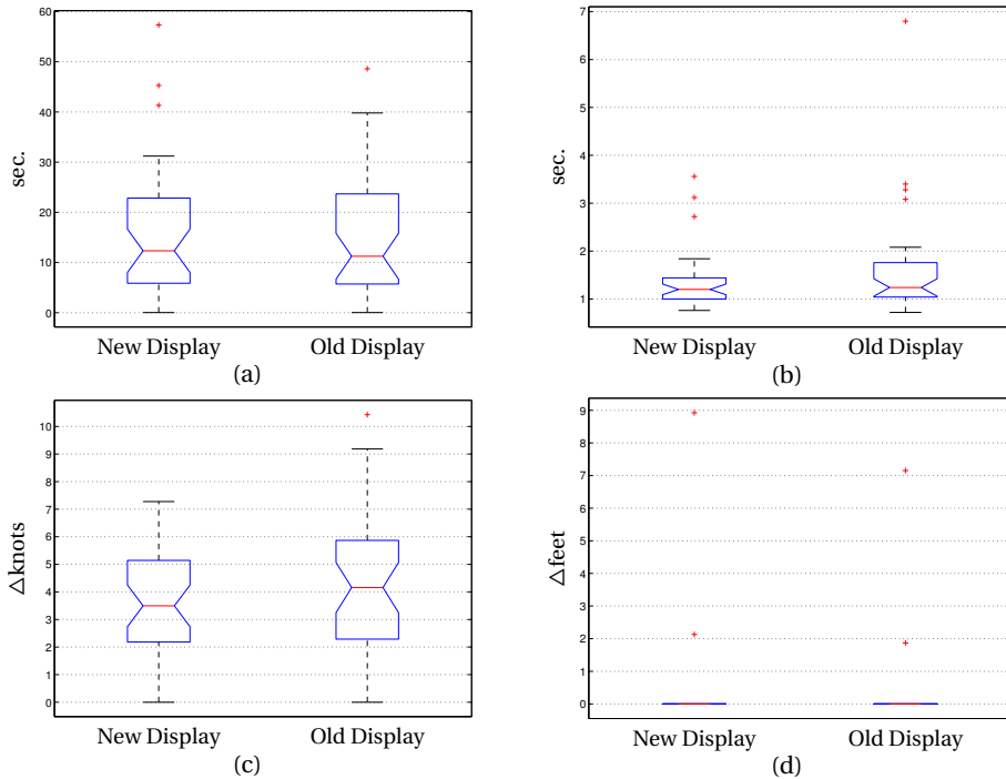
Figure 8.16: Engine Failure after take off (EFATO) , results of different display types over all runs. (a) the needed recovery time to velocity >88 KIAS, (b) the time required to achieve full rudder, (c) the maximum airspeed loss in knots and (d) the altitude loss if present.
