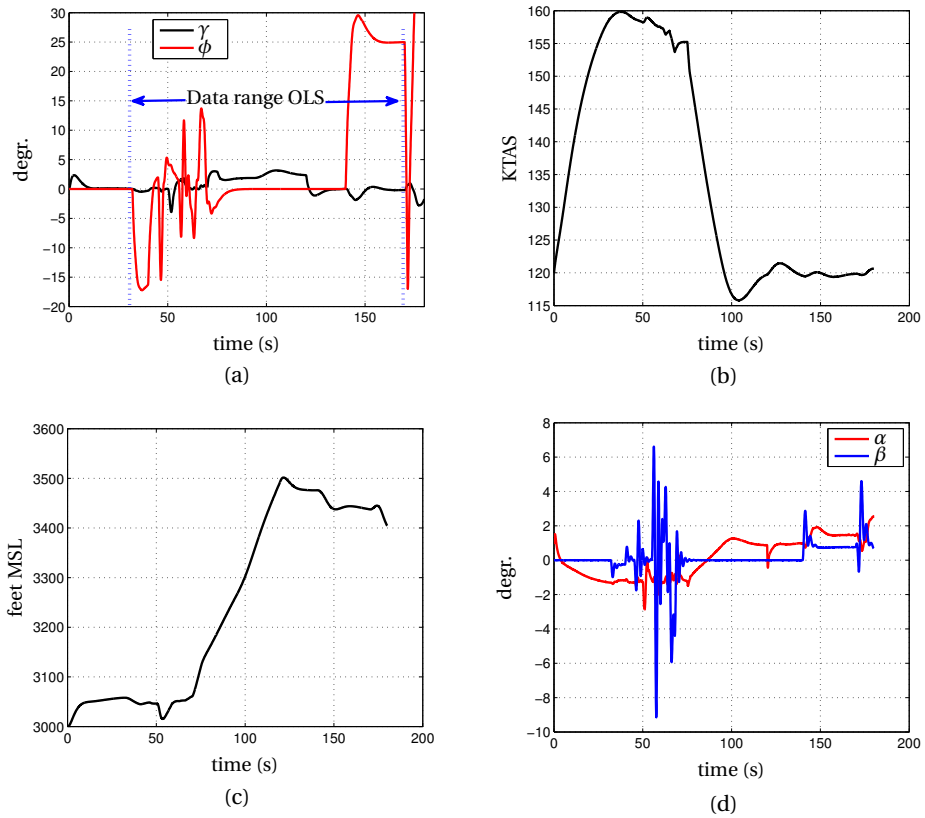
Figure 5.2: Flight profile used, failure injected at 30 seconds and maximum deflection roll at 170 seconds; (a) roll angle and climb angle (b) KTAS (c) Altitude (feet) (d) \alpha and \beta in degrees. The run is a 50% aileron failure, in smooth flying conditions with a single set of inputs.
