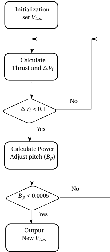
Figure B.1: The flow diagram of the propeller performance program.
