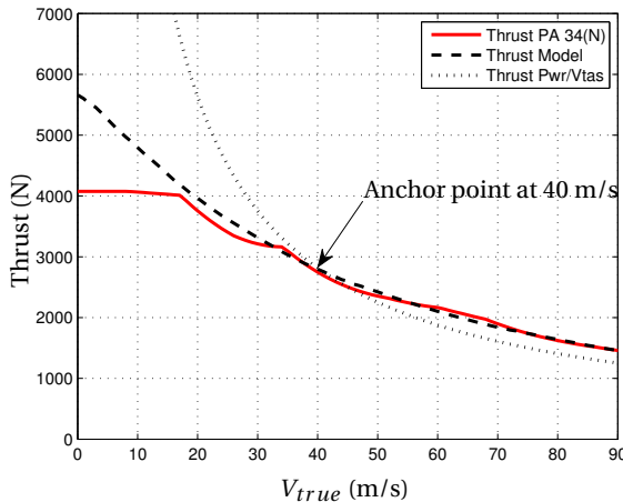
Figure A.1: Thrust of a PA-34; Comparing three models: the non-linear model based on [2], the blade model (Appendix B) and the \frac{P}{V_{true}} approximation from [1, p. 458].
