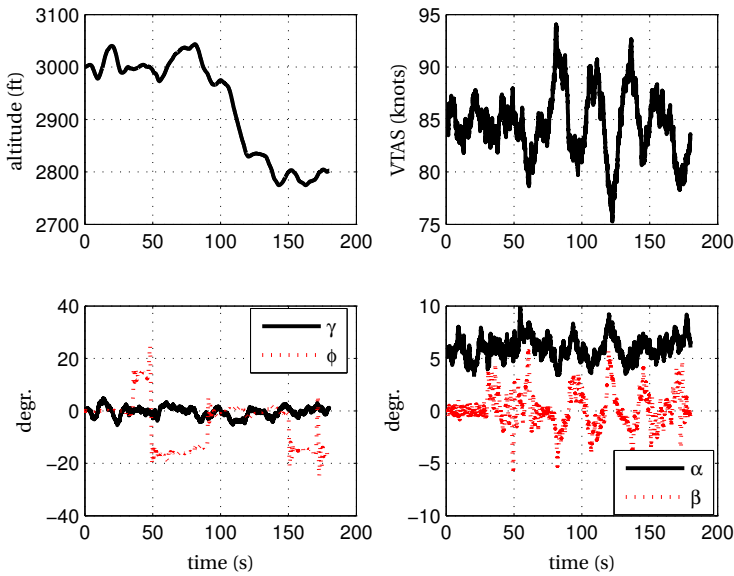
Figure 6.4: Flight profile for determining initial model parameter values. Shown profile is a left engine failure in turbulent conditions at an average true airspeed of 85 knots.
