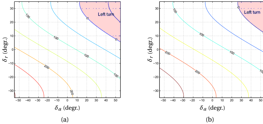
Figure 3.4: Effect of airspeed on roll performance; Available initial roll rate acceleration in \text{deg./s}^2 , for PA-34 with gear and flaps up. Left engine maximum power right engine feathered. (a) 85 KTAS, (b) 80 KTAS.
