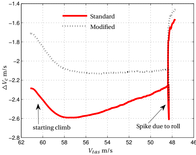
Figure 6.10: Engine failures, error in V_c comparing the normal and modified normalization for the model with 10 variables; Right engine failure in smooth flying conditions. The 'spike' at low airspeed is caused by the roll carried out at that speed.
