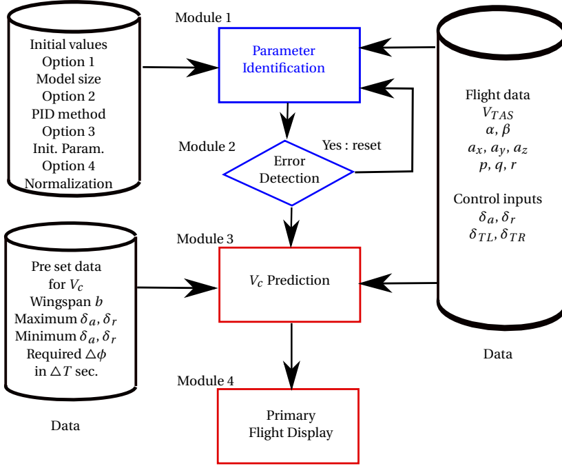
Figure 6.1: Graphic representation of the VPS. The black boxes contain the initial parameter values and flight information used. The blue boxes contain the chosen PID system and error detection system. The red boxes include the models designed in this thesis.
