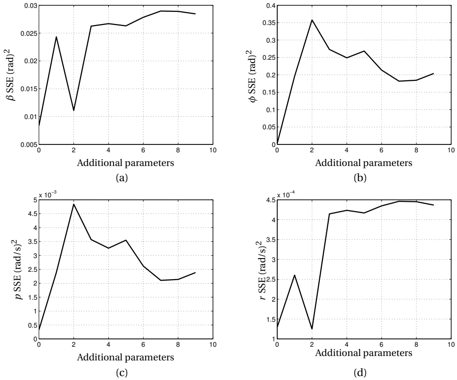
Figure 5.9: SSE error in final roll as function of added model parameters in run 181, lateral asymmetry in turbulent flying conditions; (a) \beta , (b) \phi , (c) p , and (d) r .
