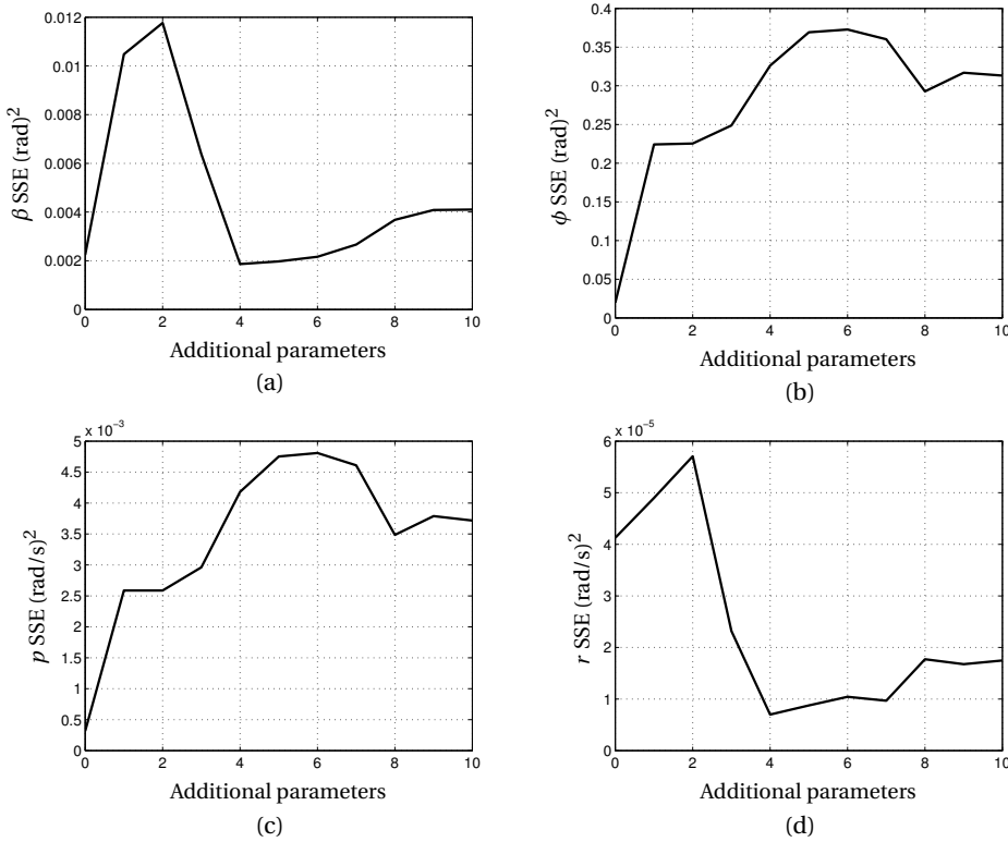
Figure 5.8: SSE error of \beta , \phi , p and r , in the final roll manoeuvre, as function of added model parameters; shown is run 177, a lateral asymmetry in smooth flying conditions.
