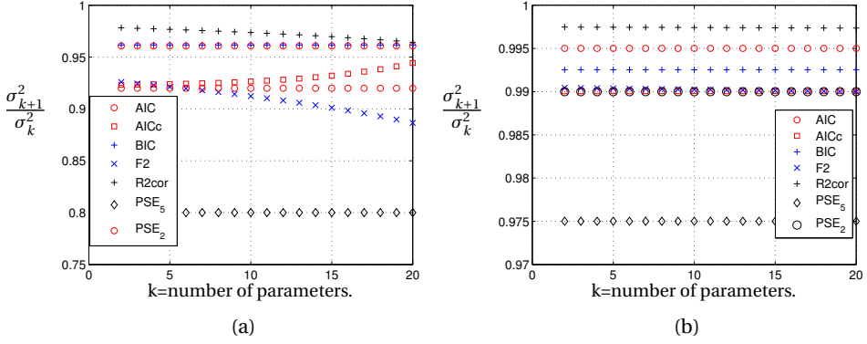
Figure 5.6: Comparing the different model selection criteria for (a) N=50 and (b) N=400
