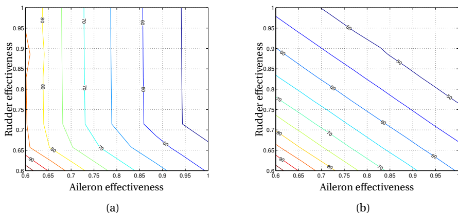
Figure 4.1: Effect of rudder effectiveness levels combined with and right engine failure on V_c (KTAS) (a) V_{c1} and (b) V_{c2} .
