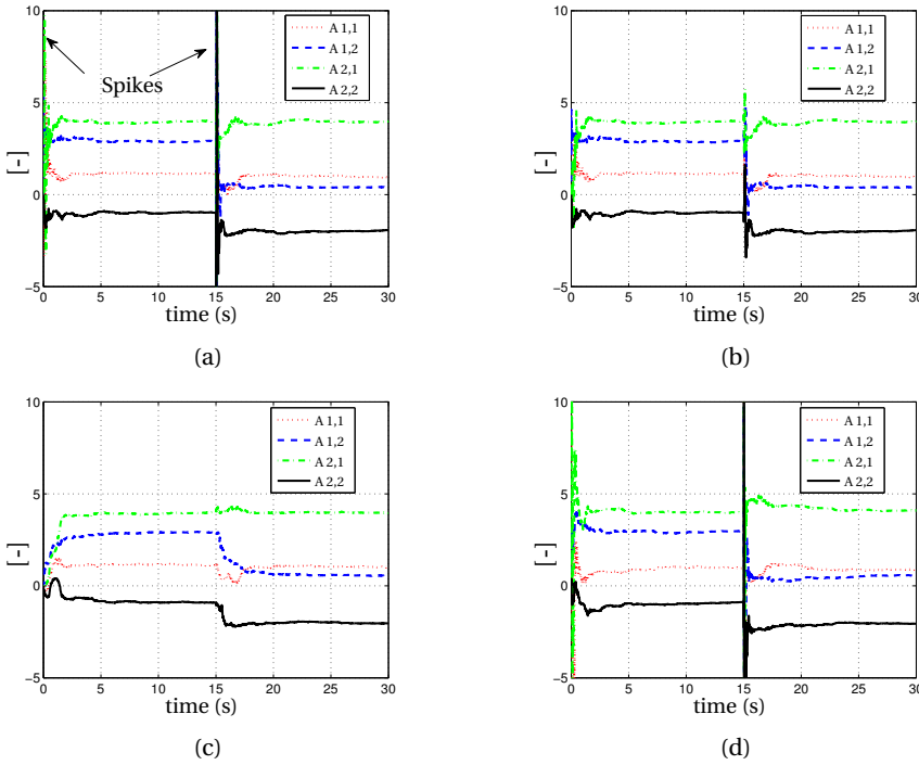
Figure 6.2: Comparison of RLS and MKM PID method when system A changes at 15 sec. in a high noise environment S/N=0.5 . In (a) RLS response; in (b) MKM with adaptive R ; in (c) MKM with very large R , which causes heavy damping and in (d) MKM with small R that becomes identical to RLS.
