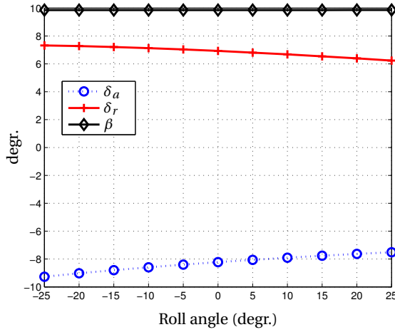
Figure 3.9: Required aileron and rudder deflection to maintain a level turn with 10^\circ \beta for a PA-34 80 KTAS.
