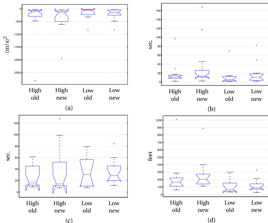
Figure 8.10: Efficiency related parameters in OEI go-around. (a) Minimum specific energy since engine failure, (b) Time minimum energy is reached after the engine failure (c) the recovery time and (d) the maximum altitude loss after the engine failure.
