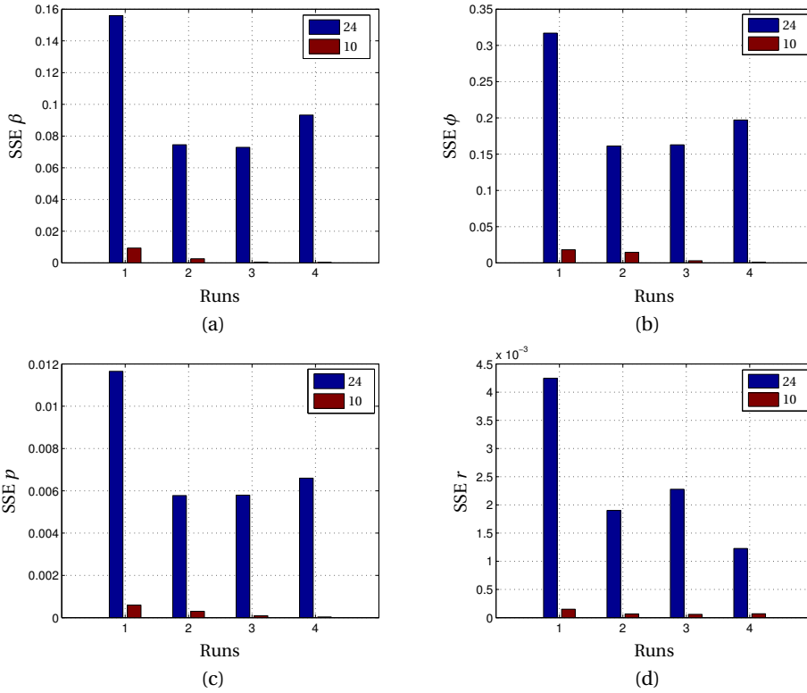
Figure 5.13: Difference in SSE of the predicted roll for both the 10 and 24 parameter model.
