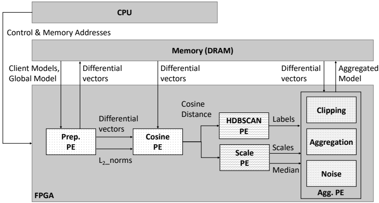
Figure 5.3: System Architecture of FLAIRS
