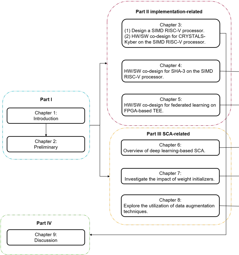
Figure 1.1: Thesis Outline.
