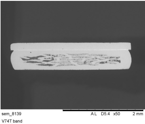
Figure 2.11: Cross-section of a single MgB 2 wire used in this thesis.
