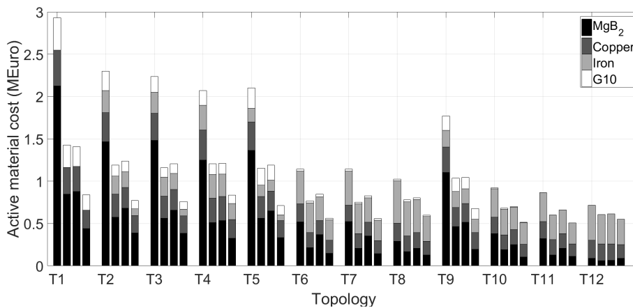
Figure 3.20: Comparison of active material costs for twelve topologies. From the left to right within a topology are original case, Scenario 1, Scenario 2 and Scenario 3.
