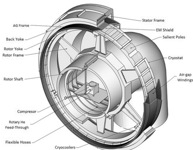
Figure 2.28: Integration concept from the Suprapower project for a 10 MW direct-drive \text{MgB}_2 generator. Patented by Tecnalia. [98]
