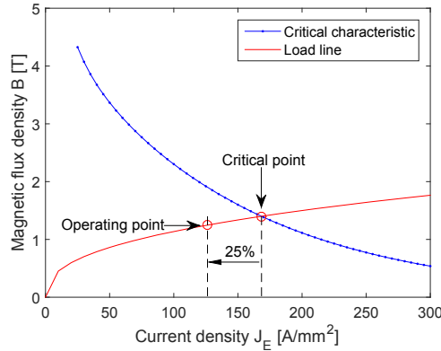
Figure 3.8: Definition of the operating point of the field current density by crossing the load line and the critical characteristic at the temperature of 20 K.
