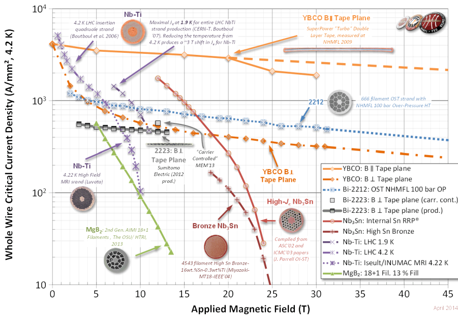
Figure 2.6: Critical characteristics of different superconductors at 4.2 K. Bi-2212 and Bi-2223 are both 1G HTS (BSCCO) with different wire architectures. YBCO is 2G HTS (ReBCO). B \perp and B \parallel are the magnetic fields perpendicular and parallel to the longer side of a superconductor (tape plane), respectively. LHC stands for large hadron collider. MRI stands for magnetic resonance imaging. Reproduced from [46].
