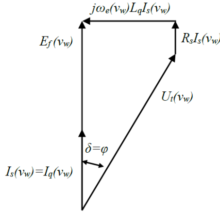
Figure 3.13: Phasor diagram of the generator operating point.
