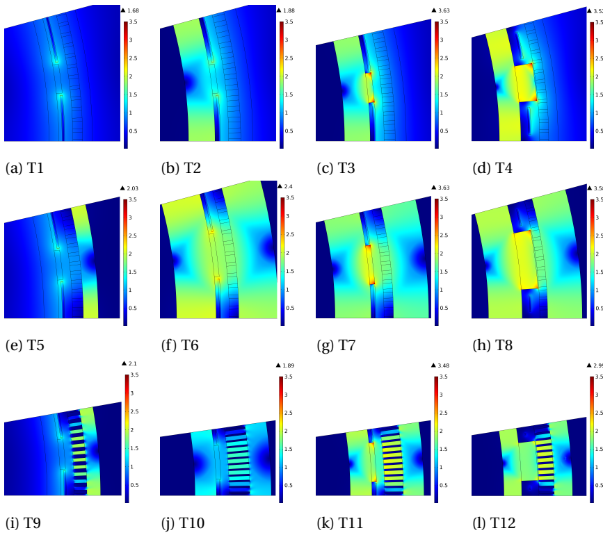
Figure 3.17: One pole of the optimized geometry and the corresponding distribution of magnetic flux density of the twelve optimized topologies in the original case (current unit cost and current density capability of the \text{MgB}_2 wire).
