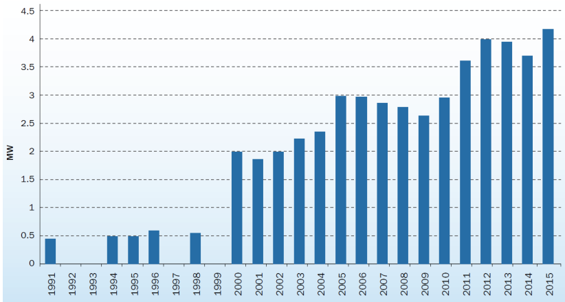
Figure 1.2: Average power rating of offshore wind turbines newly installed per year in Europe. [7]
