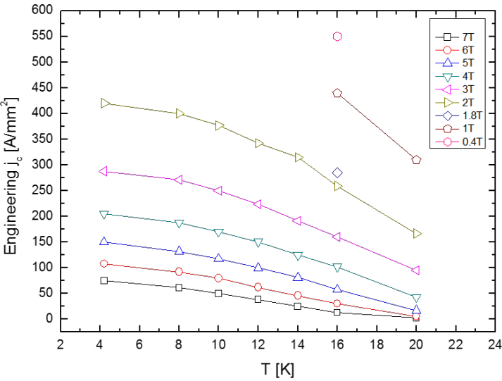
Figure 2.12: Critical characteristics of the employed MgB 2 in the J - T plane.
