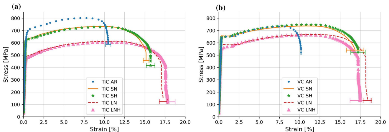
Figure 10 Representative Slow Strain Rate Tensile (SSRT) curves for all conditions in a the TiC alloy and b the VC alloy. Error bars show standard deviations in the fracture strain [%].
