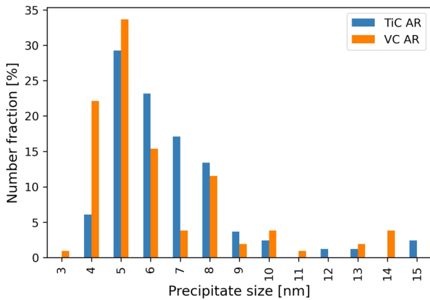
Figure 2 Normalised TiC and VC precipitate size distributions in the AR alloys. Sizes are the average ( \sqrt{\text{length} \times \text{width}} ) sizes of platelet-shaped precipitates.
