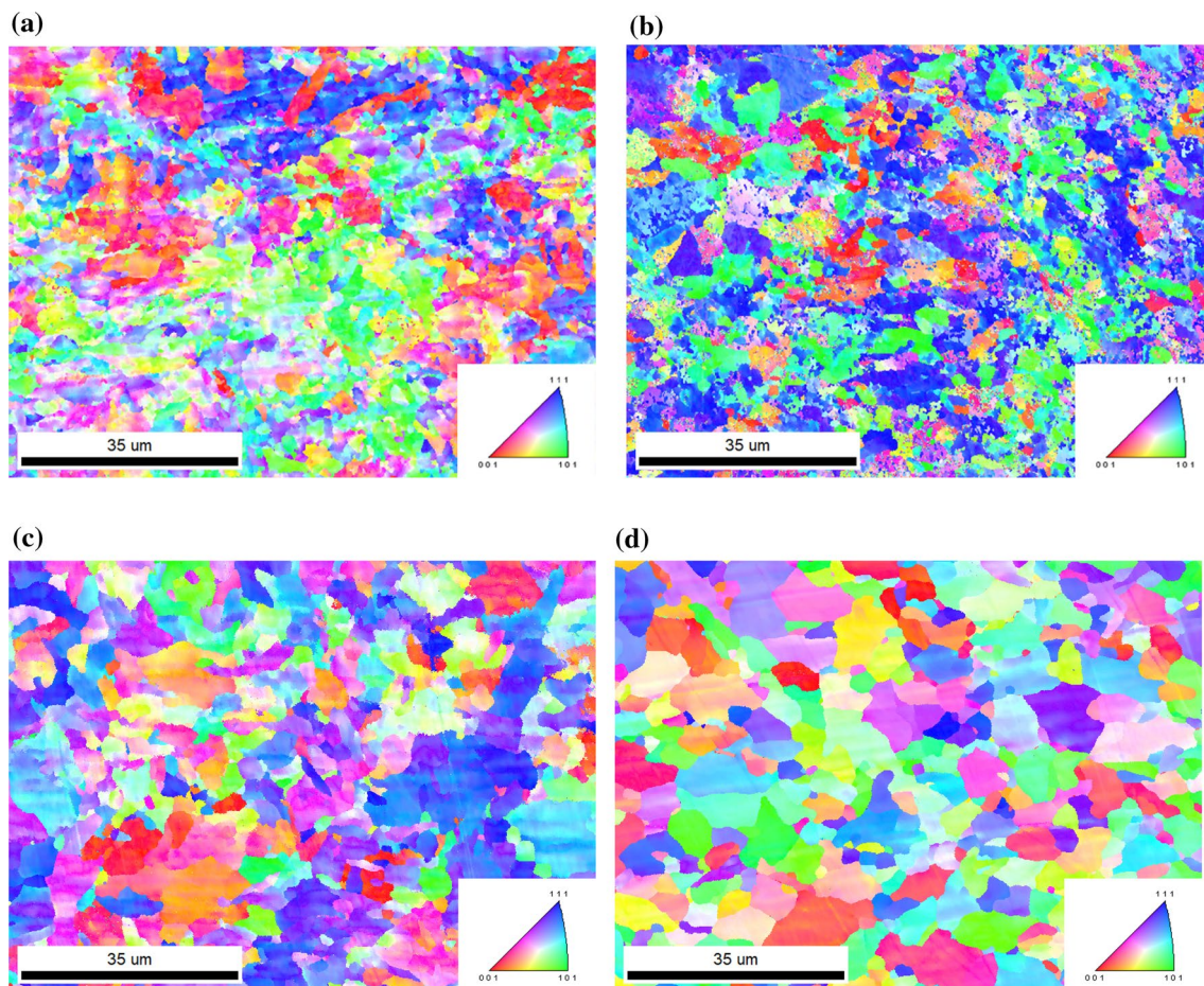
Figure 4 Inverse pole figures of the a \text{TiC}_{\text{SN}} , b \text{TiC}_{\text{LN}} , c \text{VC}_{\text{SN}} and d \text{VC}_{\text{LN}} conditions, obtained using the OIM Analysis™ software.
