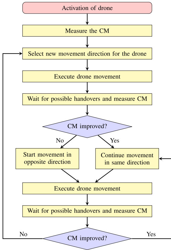
Fig. 6. Flowchart of the algorithm.
