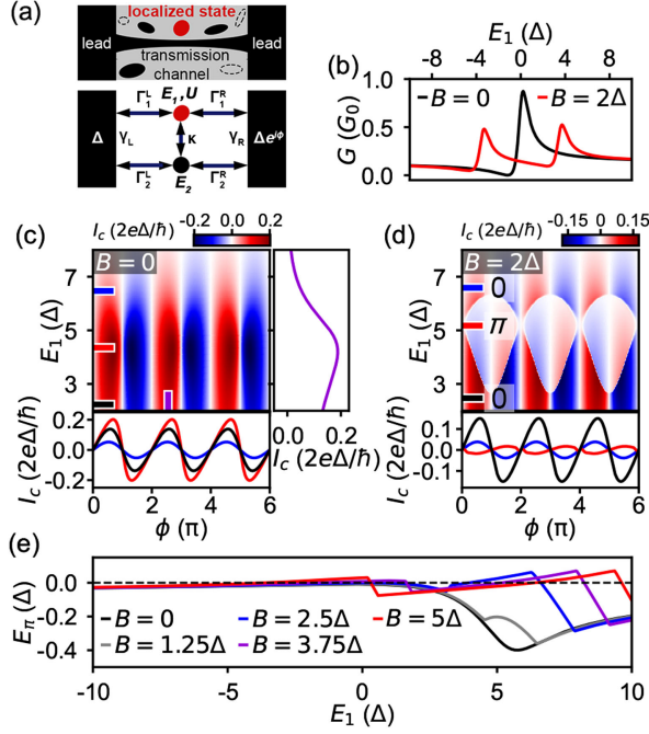
FIG. 4. (a) Schematic of the electron distribution in a nanowire JJ (top). Schematic of the two-dot model: the red dot (energy E_1 , charging energy U ) and the black dot (energy E_2 , no charging energy) (bottom). Tunneling couplings to the leads (left, right) and between the dots are taken in ratios \Gamma_1^L:\Gamma_1^R:\kappa = 0.001:0.001:1 and \Gamma_2^L:\Gamma_2^R:E_2 = 0.33:0.67:1.2 . (b) G as a function of E_1 for B = 0 (black) and B = 2\Delta (red). (c) I_c (units 2e\Delta/\hbar ) as a function of \phi and E_1 for B = 0 . Horizontal line cuts (blue, red, and black) are shown below, and a vertical line cut (purple) is shown on the right. (d) Analogous to (c), but for B = 2\Delta . (e) E_\pi as a function of E_1 for different B . In (b)–(e), the charging energy is neglected by taking U = 0 .
